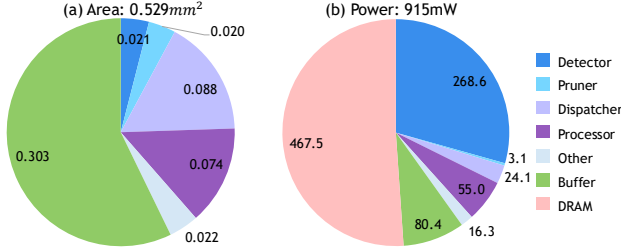
Fig. 10. Prosperity area and power breakdown.
