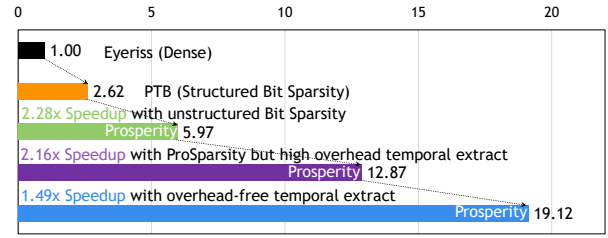
Fig. 9. Ablation study of Prosperity .
