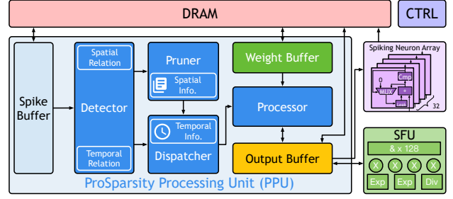
Fig. 4. Overview of Prosperity architecture.
