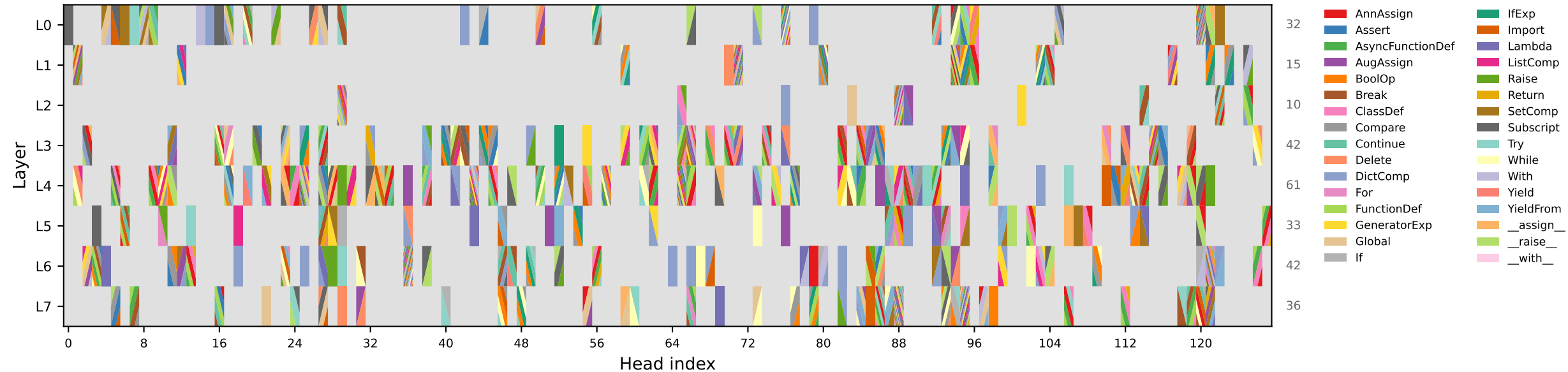
Attention head ownership by AST class (grey = below SEL threshold=0.4) — diagonal strips = multi-owned (218/271 polysemantic)
