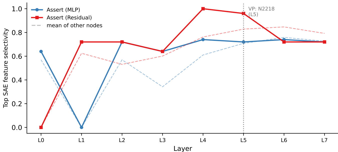
(a) Assert SAE selectivity profile (VP: monosemantic MLP neuron at L5)
