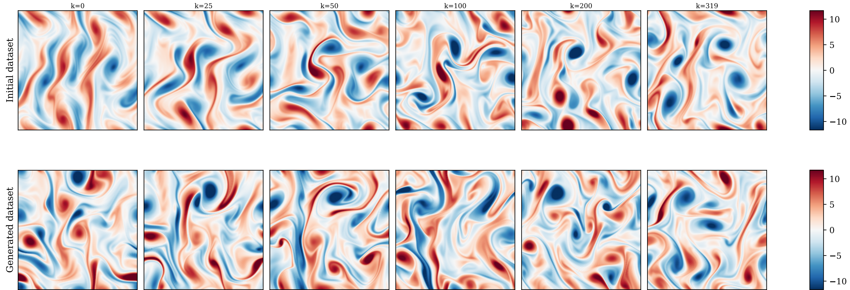
Dataset sample trajectory vorticity fields
