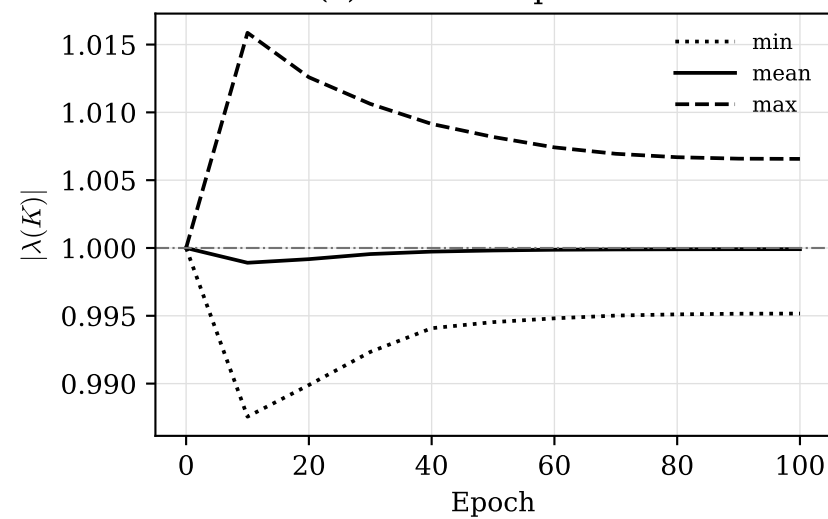
(c) Forward spectrum
