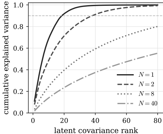
cumulative spectrum
