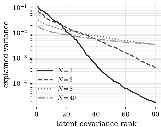
covariance spectrum
