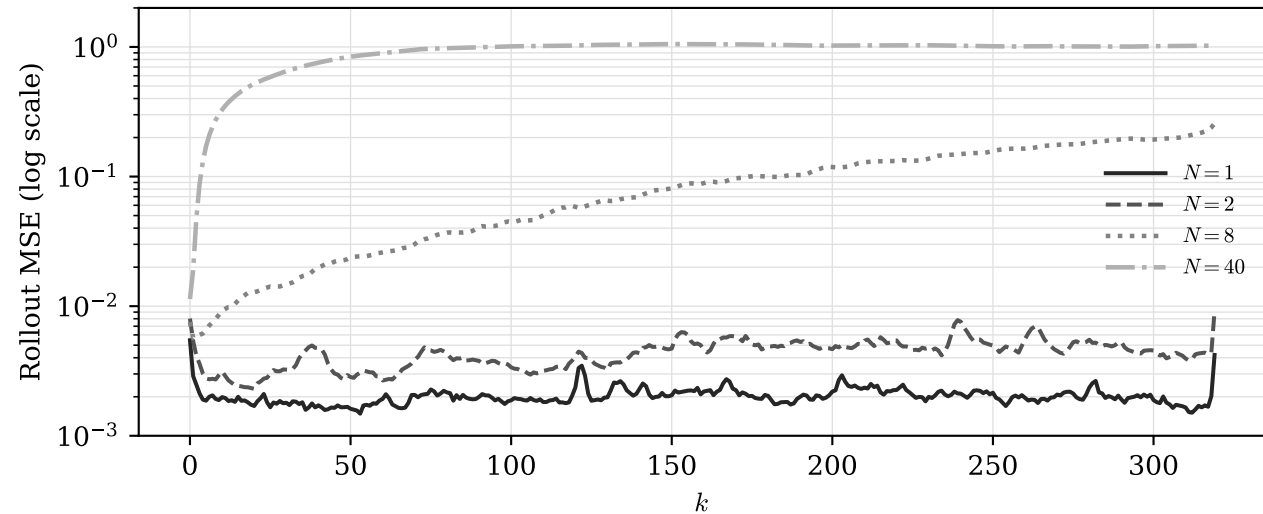
Least-squares latent linearizability probe
