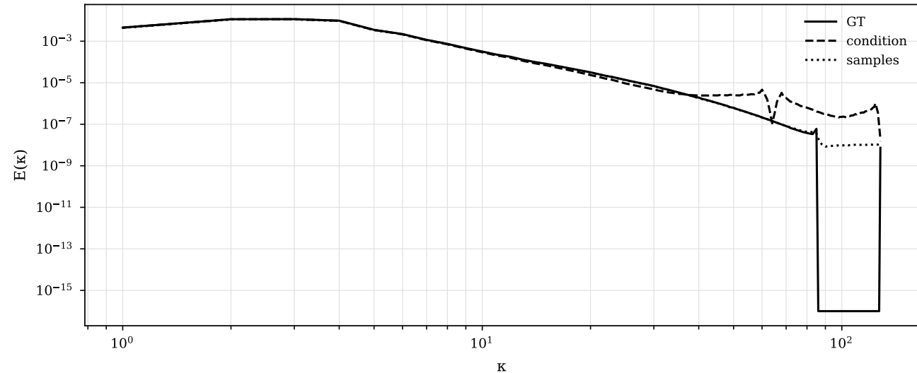
SR reconstruction energy spectrum
