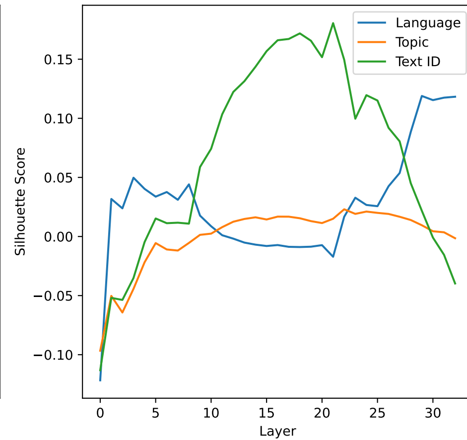
Sailor2-8B
