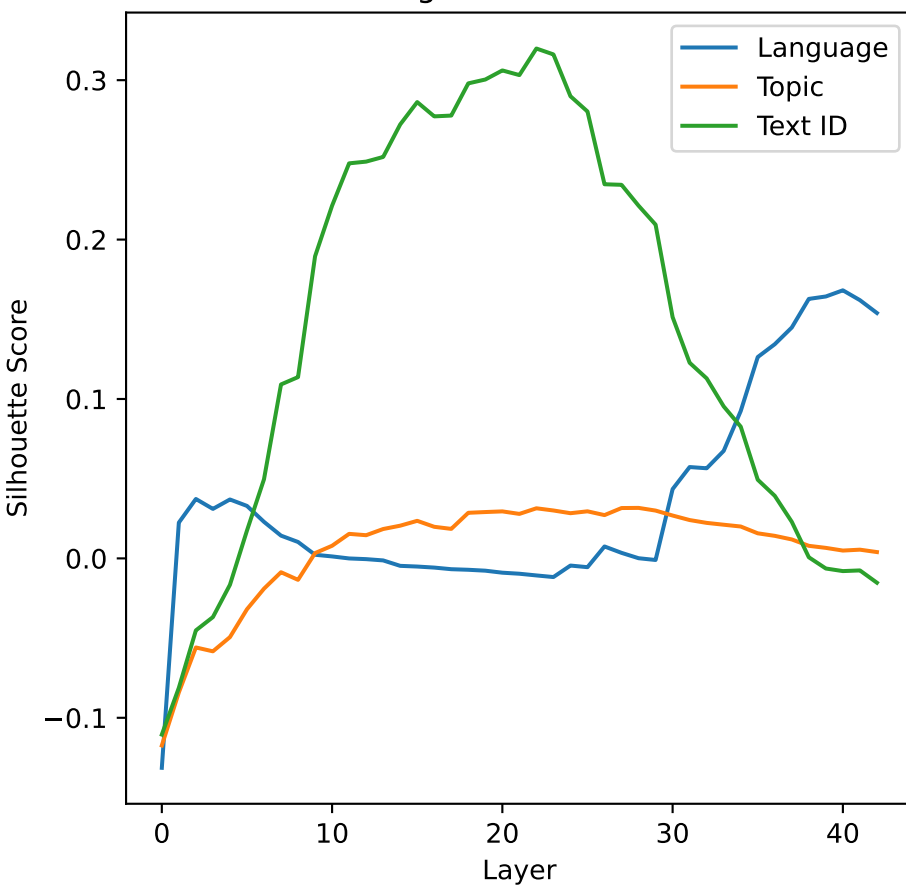
Llama-SEA-LION-v3-8B
