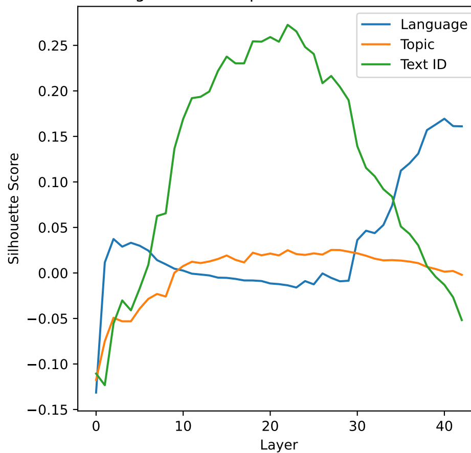
Qwen2.5-7B
