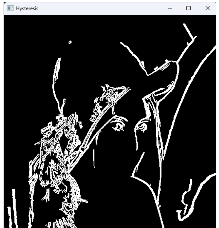
Fig 2.6: Hysteresis Thresholding
