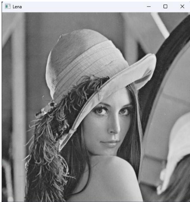
Fig 2.1: Original Image
