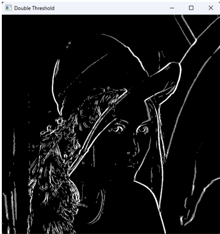
Fig 2.5: Double Thresholding
