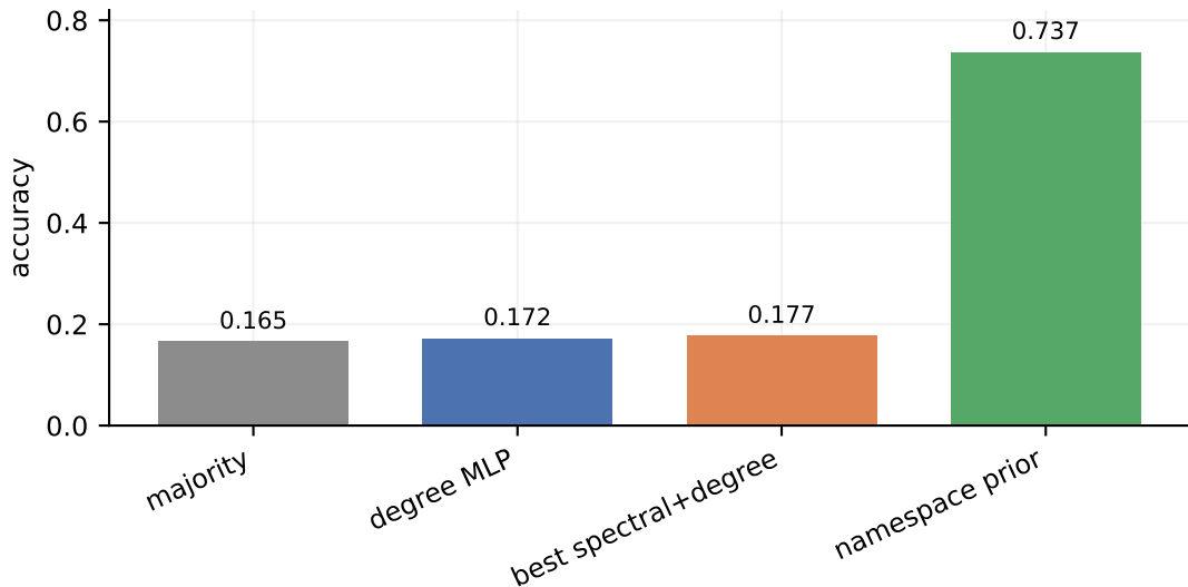
Top-level Mathlib area prediction
