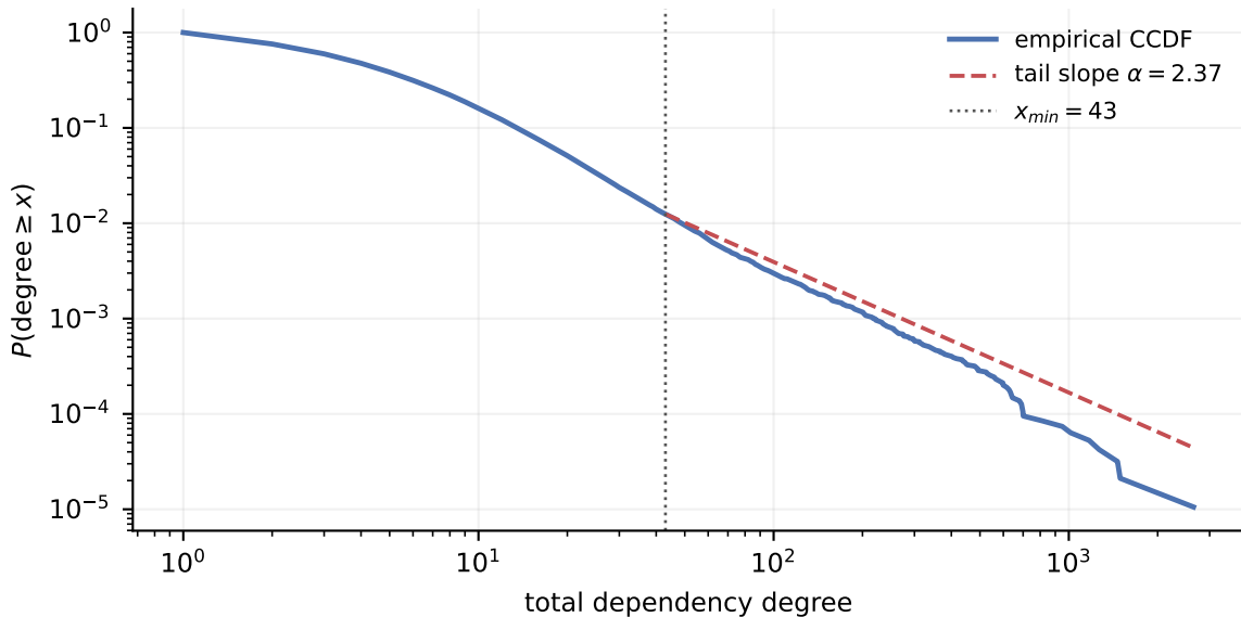
Heavy-tailed dependency-degree distribution
