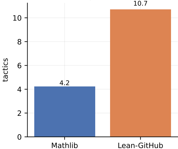
Mean proof length
