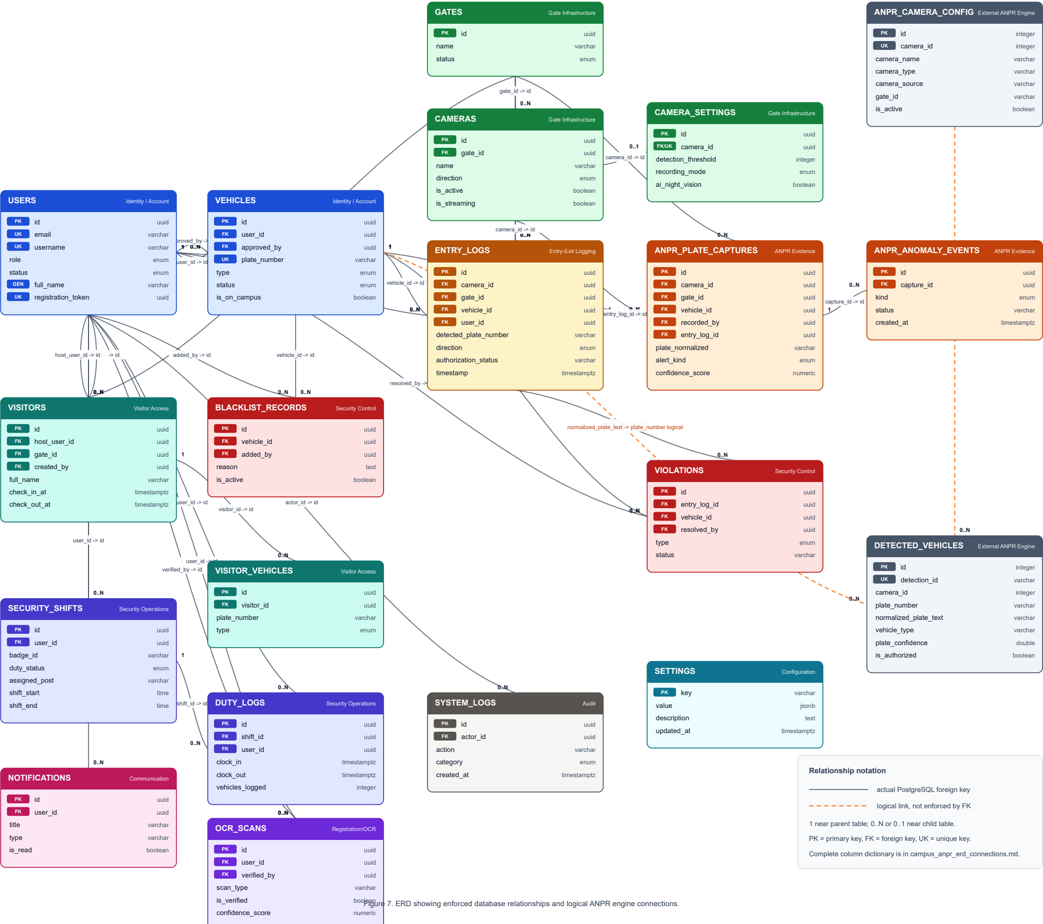
Figure 7. Entity-Relationship Diagram: Actual Table Connections
