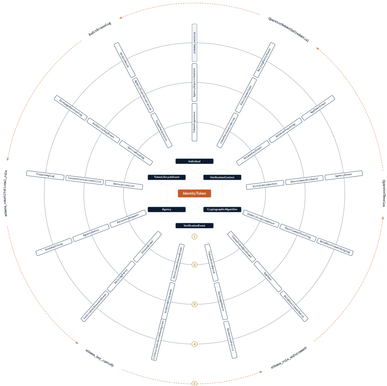
Figure 4: The 45 canonical tables of 01_schema.sql at 1.0.0-rc.7, as rings around the nucleus. The faint lattice at the centre is the nucleus geometry of Figure 2 at the same proportions. Ring two is the credential machinery: signatures, permissions, epochs, recovery, duress, the holder’s key, the card. Ring three is authority, trust and the people at the counter: who may sign under which algorithm, who trusts whom, revocation ceilings, quotas, relying parties, the replay registers, and what an enrolment rested on. Ring four is the archives, watchtowers and decisions kept as records: append-only logs, anchors, the retention decision as data, and the events that record every change to an authority, an operator account or a relying party. A migrated deployment holds seven more tables, drawn dashed: the migration registry closes the fourth ring, so rings two, three and four have the same thirteen spokes, and the other six (operator sessions, their hardware keys, the audit-access log and Athena’s three curated tables) form a fifth, hexagonal ring that echoes the nucleus. Its arrows all turn one way: migrations applied one after another, round the canonical schema. The five partition children are not drawn.
