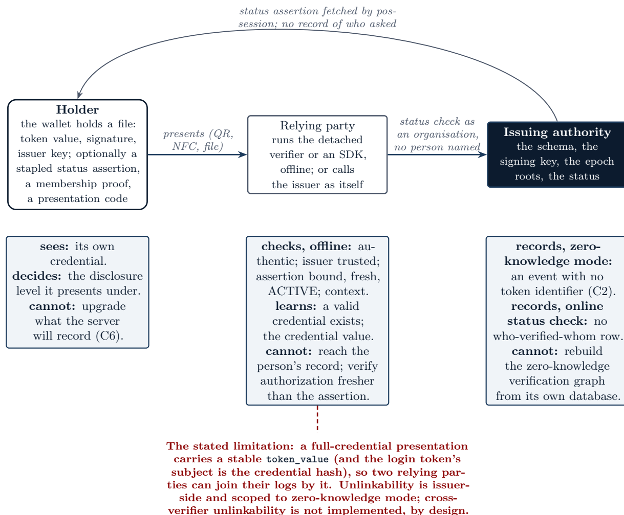
Figure 8: Holder, relying party and issuer, with what each sees and what each is prevented from seeing. The holder presents a file; the relying party decides offline with the detached verifier or an SDK and learns that a valid credential exists and its value; the issuer records, in zero-knowledge mode, an event with no token identifier, and keeps no who-verified-whom row for the online status check. The red edge is the stated limitation: on a plain presentation the credential value is a stable handle across the verifiers it is shown to.
