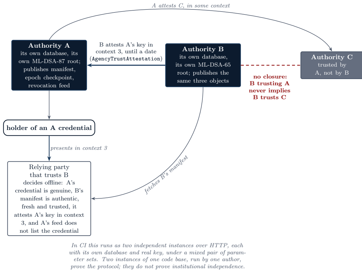
Figure 9: Two authorities and one directional attestation. B attests A's key in one context; a relying party that trusts B accepts A's credential in that context, offline, from B's manifest and A's revocation feed. A also trusts C, and that gives B nothing: trust is never a closure. In CI this runs as two independent instances over HTTP under a mixed pair of parameter sets.
