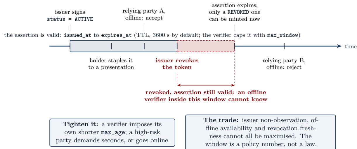
Figure 7: The offline trade, drawn as a timeline. The issuer signs a status assertion with a window; the holder staples it; a relying party verifying offline inside the window accepts. If the issuer revokes the credential inside the window, the last ACTIVE assertion stays valid until it expires, and an offline verifier cannot know. The window is bounded by the issuer's time-to-live (an hour by default) and by the max_window the verifier imposes; a high-risk relying party demands seconds or goes online.
