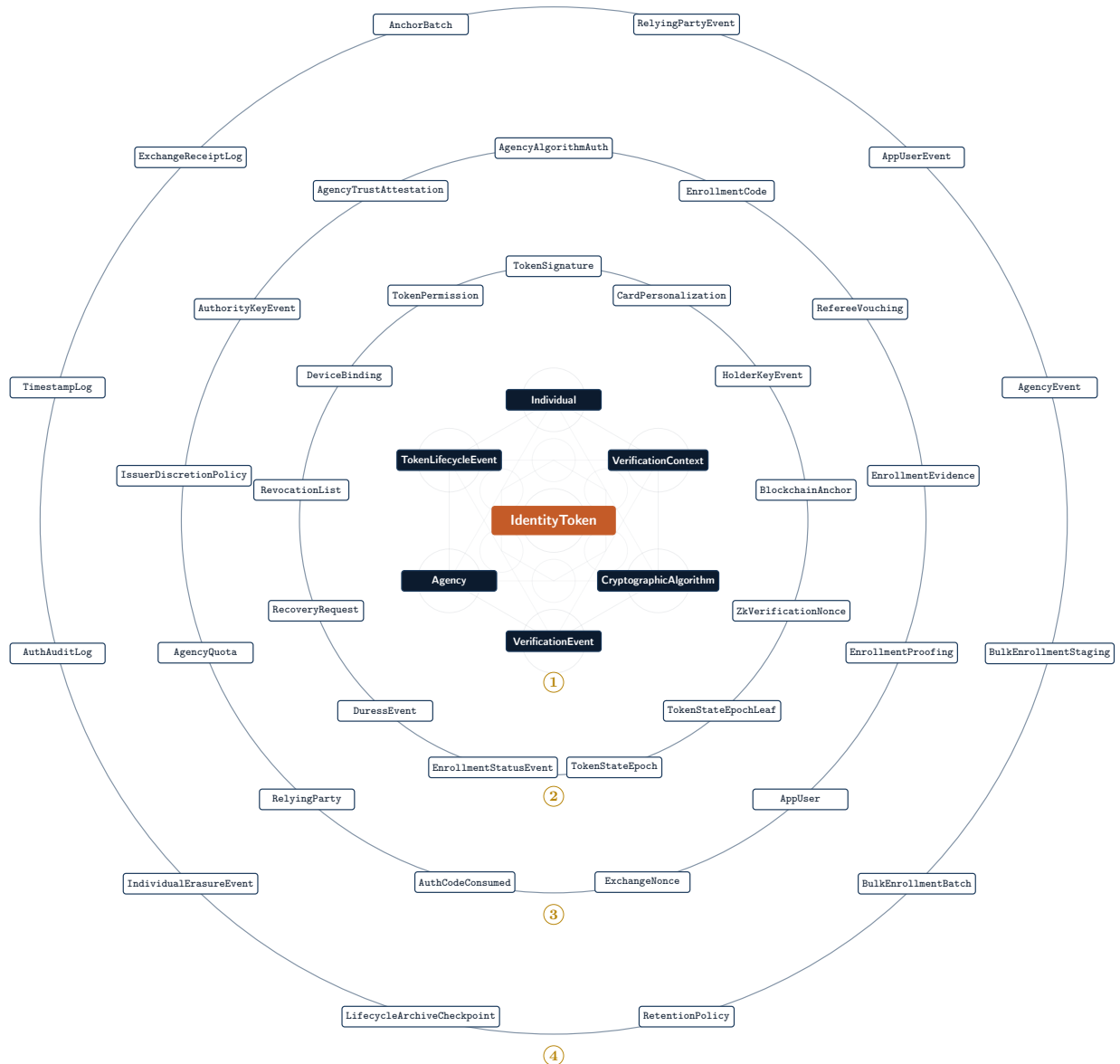
Figure 4: The 45 canonical tables of 01_schema.sql at 1.0.0-rc.1, as rings around the Version 1 nucleus. The faint lattice at the centre is the nucleus geometry of Figure 2 at the same proportions. Ring two is the credential machinery: signatures, permissions, epochs, recovery, duress, the holder's key, the card. Ring three is authority, trust and the people at the counter: who may sign under which algorithm, who trusts whom, revocation ceilings, quotas, relying parties, the replay registers, and what an enrolment rested on. Ring four is the archives, watchtowers and decisions kept as records: append-only logs, anchors, the retention decision as data, and the events that record every change to an authority, an operator account or a relying party. A migrated deployment holds seven more tables (the migration registry, operator sessions and credentials, the audit-access log, and Athena's three curated tables) and five partition children.
