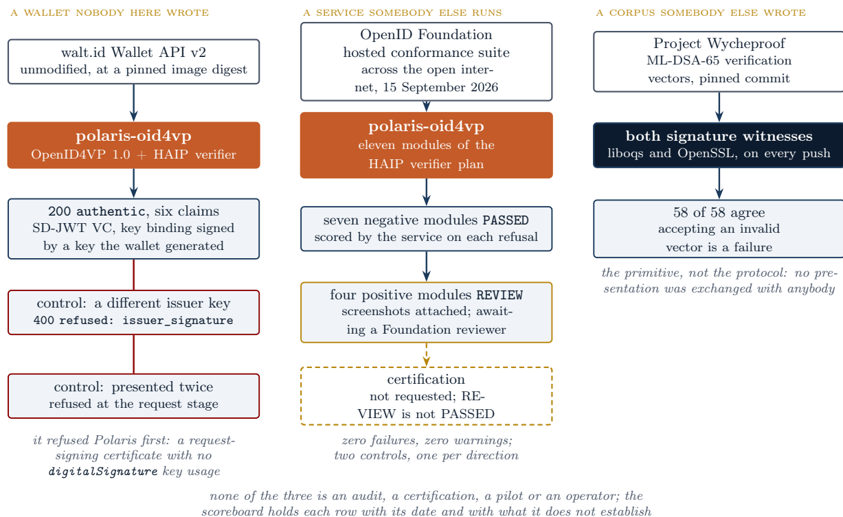
Figure 6: The three things outside the repository that have exercised it, and the two controls without which the first would mean nothing. A wallet nobody here wrote presented a credential and was accepted; the same wallet, with the verifier trusting a different issuer key, was refused; and a re-presentation against an answered request was refused. The Foundation’s hosted suite scored seven refusals itself and left four acceptances for a human reviewer. A published corpus agrees with both signature witnesses on the primitive. None of the three is an audit, a certification or a pilot.
