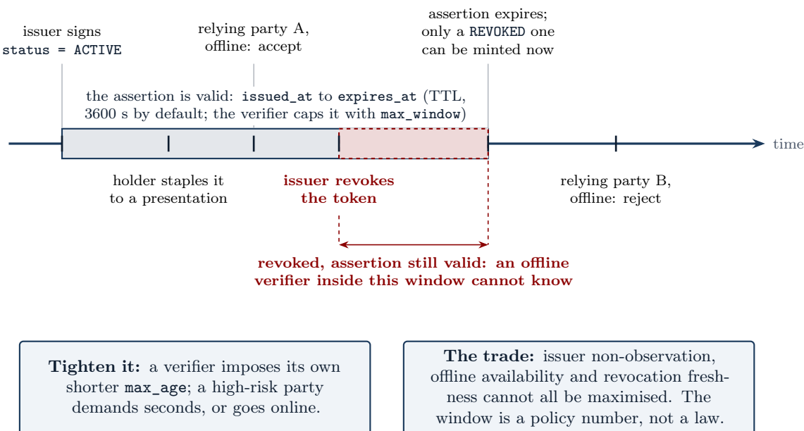
Figure 5: The offline trade, drawn as a timeline. The issuer signs a status assertion with a window; the holder staples it; a relying party verifying offline inside the window accepts. If the issuer revokes the credential inside the window, the last ACTIVE assertion stays valid until it expires, and an offline verifier cannot know. The window is bounded by the issuer’s time-to-live (an hour by default) and by the max_window the verifier imposes; a high-risk relying party demands seconds or goes online. Who chooses the window, and who bears it: the issuer sets the time-to-live and each relying party its max_window ; the harm of a long window falls on whoever relies on a credential revoked inside it, and on the holder whose revocation was meant to protect them. Polaris makes the window explicit and bounded; how long is acceptable is a governance decision it does not make.
