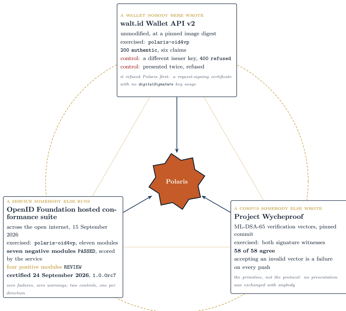
Figure 15: The three things outside the repository that have exercised it, and the two controls without which the first would mean nothing. A wallet nobody here wrote presented a credential and was accepted; the same wallet, with the verifier trusting a different issuer key, was refused; and a re-presentation against an answered request was refused. The Foundation's hosted suite scored seven refusals itself and left four acceptances for a human reviewer; a later run of the same plan was certified. A published corpus agrees with both signature witnesses on the primitive.
