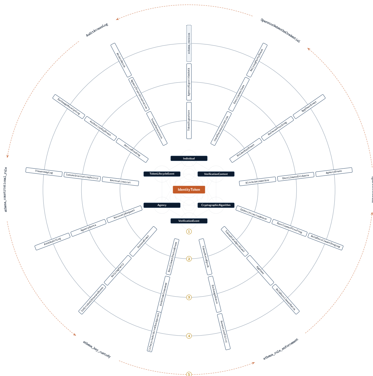
Figure 5: The 45 canonical tables of 01_schema.sql at 1.0.0-rc.7 , as rings around the nucleus. The faint lattice at the centre is the nucleus geometry of Figure 3 at the same proportions. Ring two is the credential machinery: signatures, permissions, epochs, recovery, duress, the holder’s key, the card. Ring three is authority, trust and the people at the counter: who may sign under which algorithm, who trusts whom, revocation ceilings, quotas, relying parties, the replay registers, and what an enrolment rested on. Ring four is the archives, watchtowers and decisions kept as records: append-only logs, anchors, the retention decision as data, and the events that record every change to an authority, an operator account or a relying party. A migrated deployment holds seven more tables, drawn dashed: the migration registry closes the fourth ring, so rings two, three and four have the same thirteen spokes, and the other six (operator sessions, their hardware keys, the audit-access log and Athena’s three curated tables) form a fifth, hexagonal ring that echoes the nucleus. Its arrows all turn one way: migrations applied one after another, round the canonical schema. The five partition children are not drawn.
