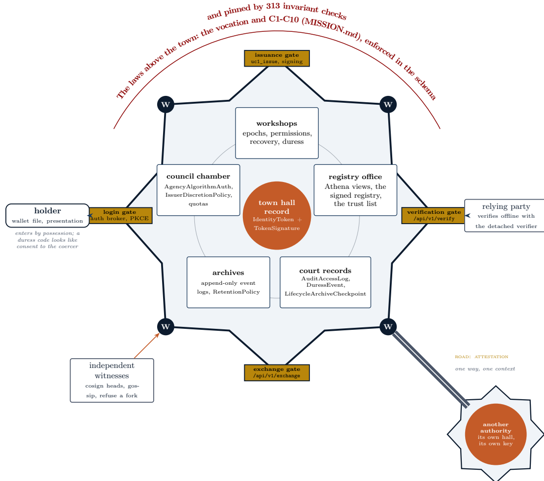
Figure 1: The walled town, with the real component beside every civic name. The register in the hall is the credential core; the wall is the schema; the four gates are the routes through which a claim enters or leaves; the watchtowers are the transparency logs and the witnesses outside the wall watch them; the road to the second town is a directional, per-context attestation; the laws above the town bind the town itself. The plan describes structure. Polaris is federated: every authority is its own town.
