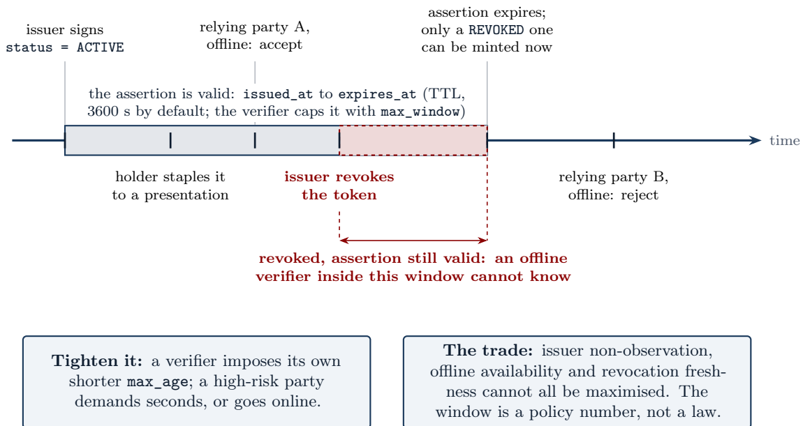
Figure 6: The offline trade, drawn as a timeline. The issuer signs a status assertion with a window; the holder staples it; a relying party verifying offline inside the window accepts. If the issuer revokes the credential inside the window, the last ACTIVE assertion stays valid until it expires, and an offline verifier cannot know. The window is bounded by the issuer’s time-to-live (an hour by default) and by the max_window the verifier imposes; a high-risk relying party demands seconds or goes online. Who chooses the window, and who bears it: the issuer sets the time-to-live and each relying party its max_window ; the harm of a long window falls on whoever relies on a credential revoked inside it, and on the holder whose revocation was meant to protect them. Polaris makes the window explicit and bounded; how long is acceptable is a governance decision it does not make.
