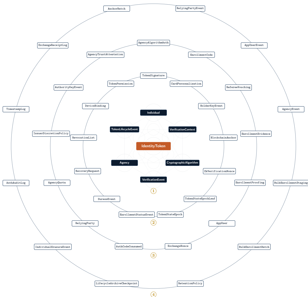
Figure 4: The 45 canonical tables of 01_schema.sql at 1.0.0-rc.1 , as rings around the Version 1 nucleus. The faint lattice at the centre is the nucleus geometry of Figure 2 at the same proportions. Ring two is the credential machinery: signatures, permissions, epochs, recovery, duress, the holder’s key, the card. Ring three is authority, trust and the people at the counter: who may sign under which algorithm, who trusts whom, revocation ceilings, quotas, relying parties, the replay registers, and what an enrolment rested on. Ring four is the archives, watchtowers and decisions kept as records: append-only logs, anchors, the retention decision as data, and the events that record every change to an authority, an operator account or a relying party. A migrated deployment holds seven more tables (the migration registry, operator sessions and credentials, the audit-access log, and Athena’s three curated tables) and five partition children.
