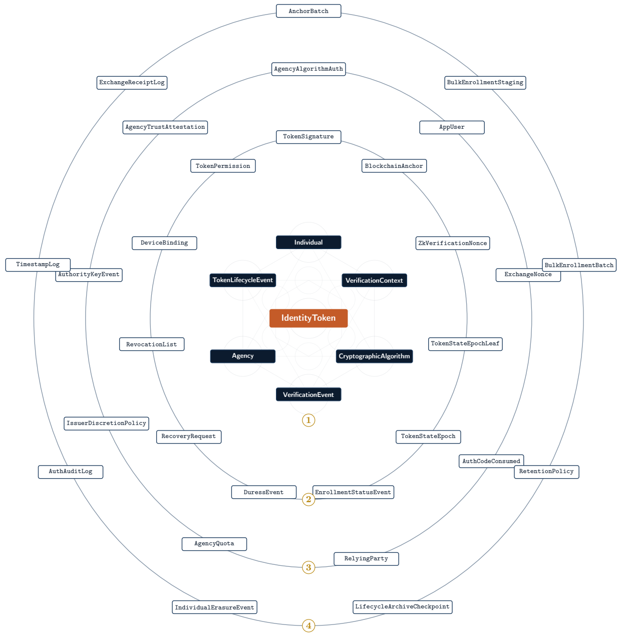
Figure 4: The 36 canonical tables of 01_schema.sql at v9.345, as rings around the Version 1 nucleus. The faint lattice at the centre is the nucleus geometry of Figure 2 at the same proportions. Ring two is the credential machinery: signatures, permissions, epochs, recovery, duress. Ring three is authority and trust: who may sign under which algorithm, who trusts whom, revocation ceilings, quotas, relying parties, the replay registers. Ring four is the archives and watchtowers: append-only logs, anchors, the retention decision as data. A migrated deployment holds seven more tables (the migration registry, operator sessions and credentials, the audit-access log, and Athena’s three curated tables), and four partition children.
