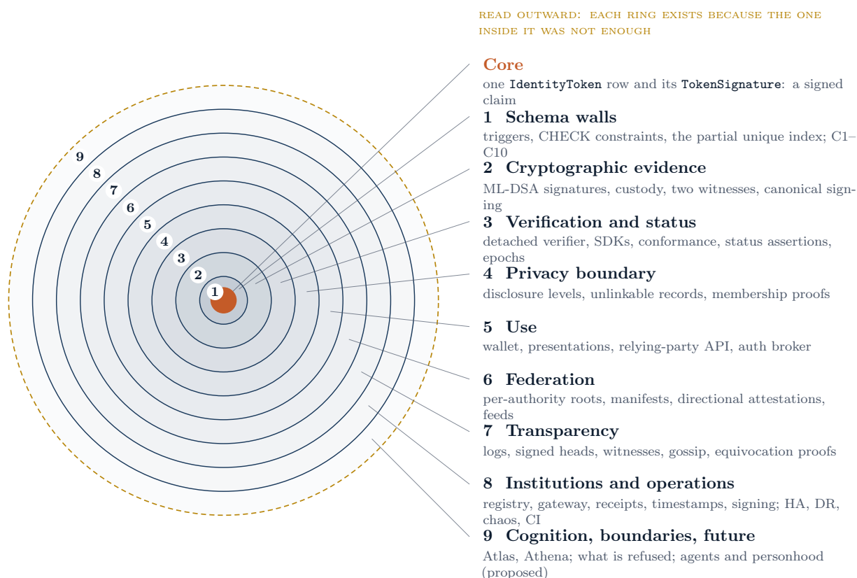
Figure 1: The concentric map of Polaris. The core is one credential record and its signature. Each ring names the actual components on it, and the reading order of the paper follows the rings outward. The outermost ring is dashed because part of it does not yet exist: cognition and boundaries are present, the agent environment is a proposal.
