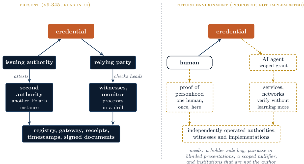
Figure 15: The present system beside the future environment it is preparation for. Solid navy is what runs at v9.345; dashed gold is what does not exist. The two panels share the same core, which is the point: the extensions are proposed on the credential and its verifiers, not on a new system.
