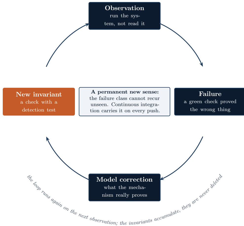
Figure 12: The loop by which an error becomes a permanent sense. Observation is running the system, not reading it; the failure is a green check that proved the wrong thing; the correction is a new statement of what the mechanism proves; the invariant is a check with a detection test; and continuous integration carries it on every push from then on.
