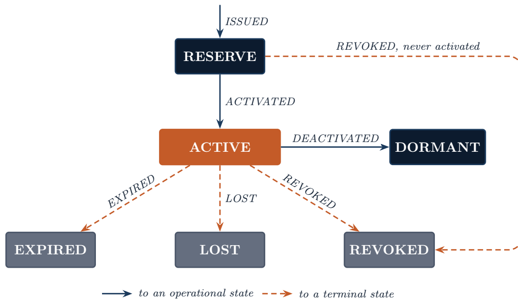
Figure 4: The token lifecycle machine as the trigger trg_token_state_machine enforces it: six legal transitions, each labelled with the lifecycle event it writes automatically. ACTIVE is the only operational state. A token enters at RESERVE and is activated, or is revoked before it ever is; an active token leaves through one of three terminal states or into DORMANT when a successor takes over.
