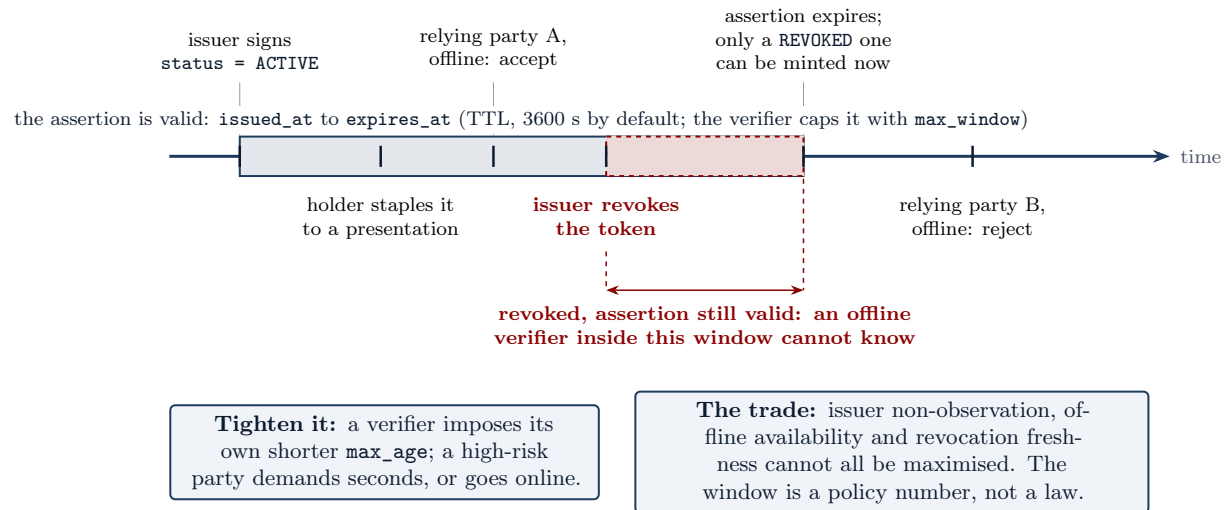
Figure 7: The offline trade, drawn as a timeline. The issuer signs a status assertion with a window; the holder staples it; a relying party verifying offline inside the window accepts. If the issuer revokes the credential inside the window, the last ACTIVE assertion stays valid until it expires, and an offline verifier cannot know. The window is bounded by the issuer’s time-to-live (an hour by default) and by the max_window the verifier imposes; a high-risk relying party demands seconds or goes online.
