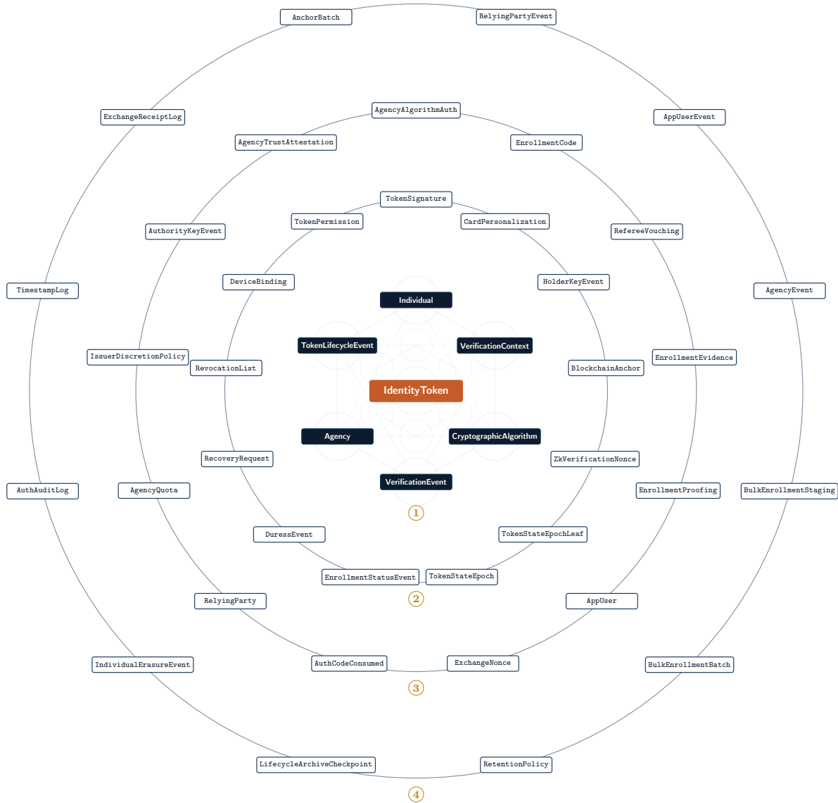
Figure 4: The 45 canonical tables of 01_schema.sql at 1.0.0-rc.7, as rings around the Version 1 nucleus. The faint lattice at the centre is the nucleus geometry of Figure 2 at the same proportions. Ring two is the credential machinery: signatures, permissions, epochs, recovery, duress, the holder's key, the card. Ring three is authority, trust and the people at the counter: who may sign under which algorithm, who trusts whom, revocation ceilings, quotas, relying parties, the replay registers, and what an enrolment rested on. Ring four is the archives, watchtowers and decisions kept as records: append-only logs, anchors, the retention decision as data, and the events that record every change to an authority, an operator account or a relying party. A migrated deployment holds seven more tables (the migration registry, operator sessions and credentials, the audit-access log, and Athena's three curated tables) and five partition children.
