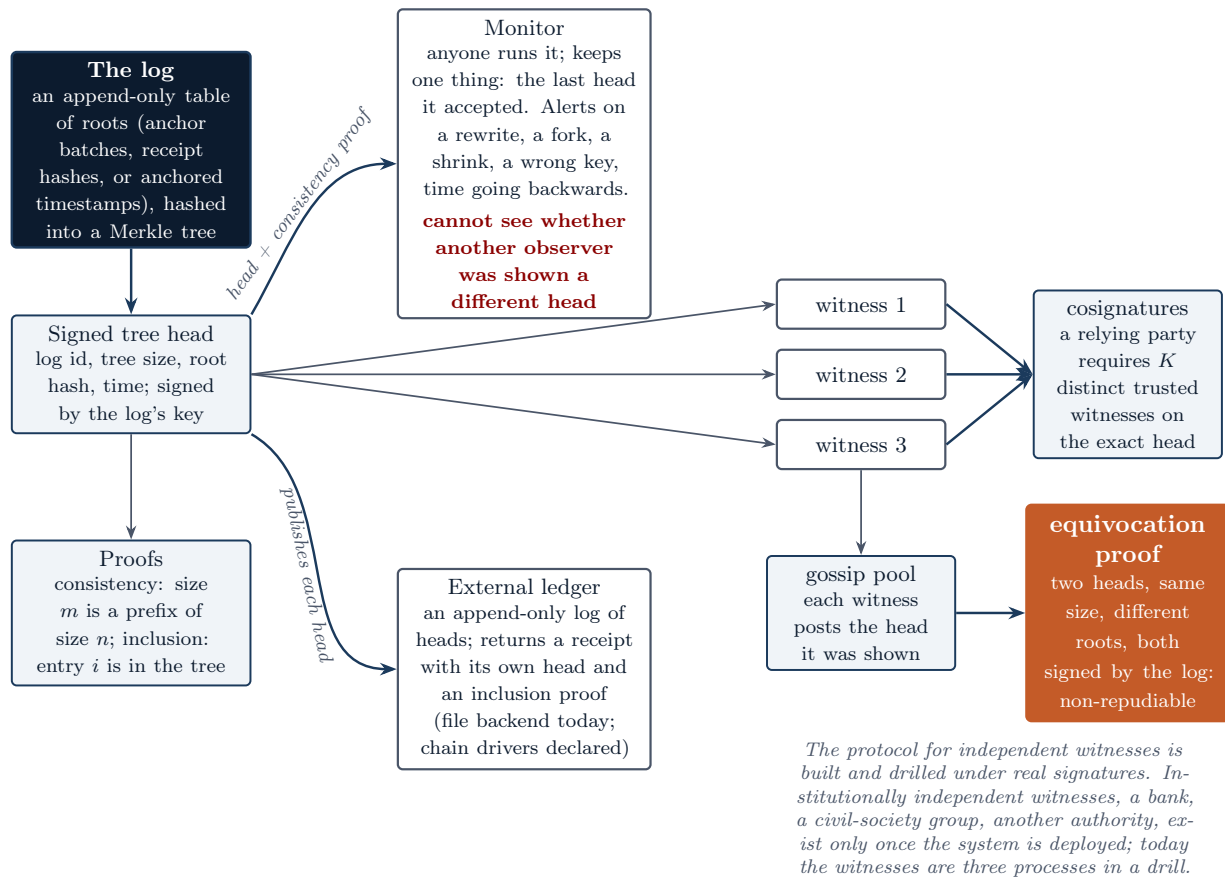
Figure 10: The log, the monitor, the witnesses, the gossip pool and the equivocation proof. The log publishes a signed head and proofs. A monitor proves the log only appended. Witnesses cosign heads they found consistent, a relying party requires a threshold of them on the exact head, and witnesses gossip the heads they were shown; two log-signed heads of the same size with different roots are a non-repudiable proof that the log lied. Heads can also be published into an external append-only ledger that returns a receipt.
