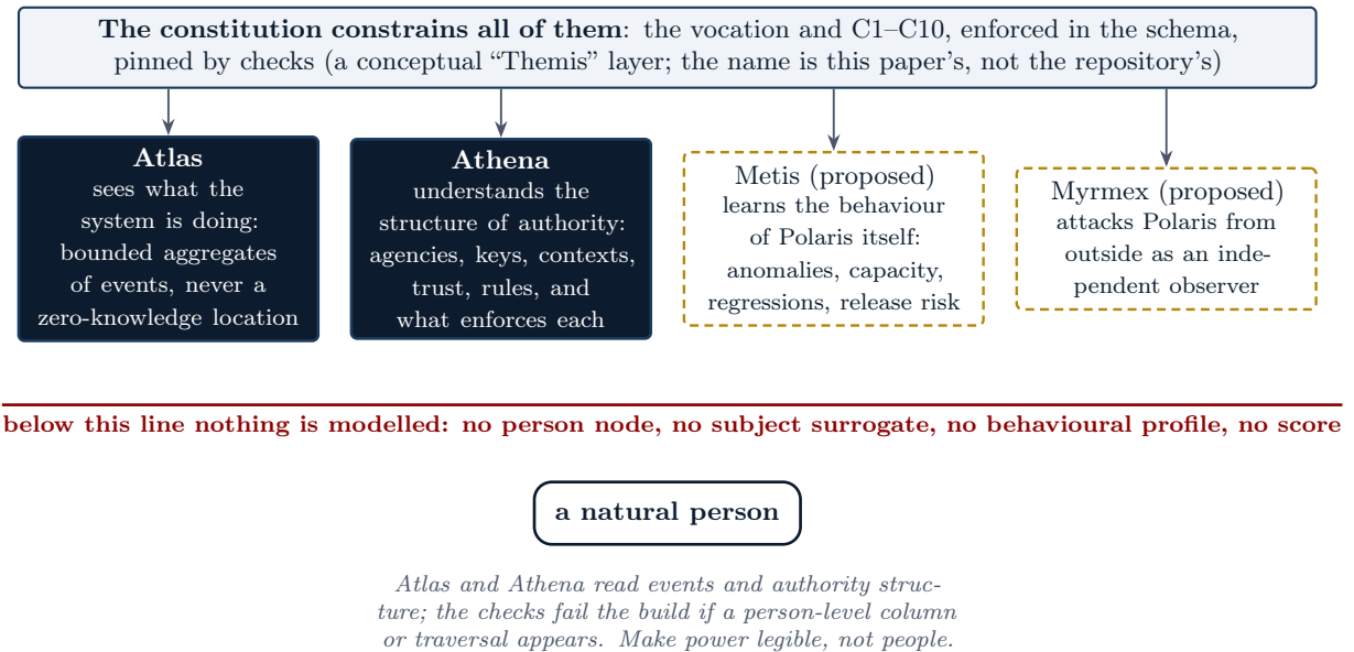
Figure 12: The cognitive layers. Atlas sees what the system is doing; Athena understands the structure of authority; Metis, proposed, would learn the behaviour of Polaris itself; Myrmex, proposed in this paper, would attack it from outside. The constitution constrains all of them. The red line is the person-prohibition: nothing above it models a natural person, and five checks fail the build if a person-level column or traversal appears in the authority layer.
