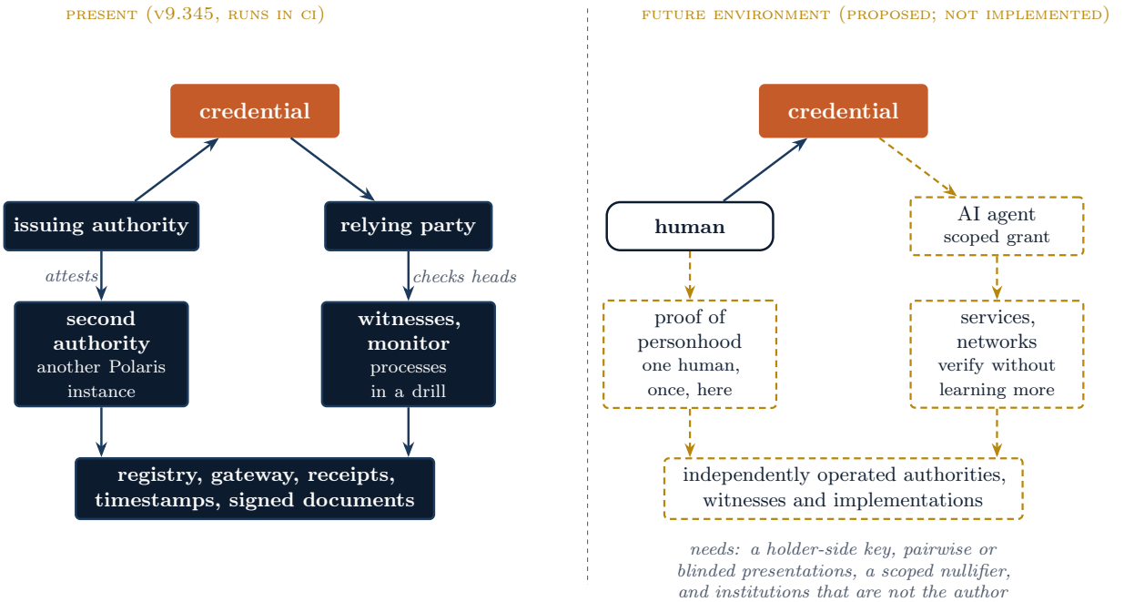
Figure 15: The present system beside the future environment it is preparation for. Solid navy is what runs at v9.345; dashed gold is what does not exist. The two panels share the same core, which is the point: the extensions are proposed on the credential and its verifiers, not on a new system.
