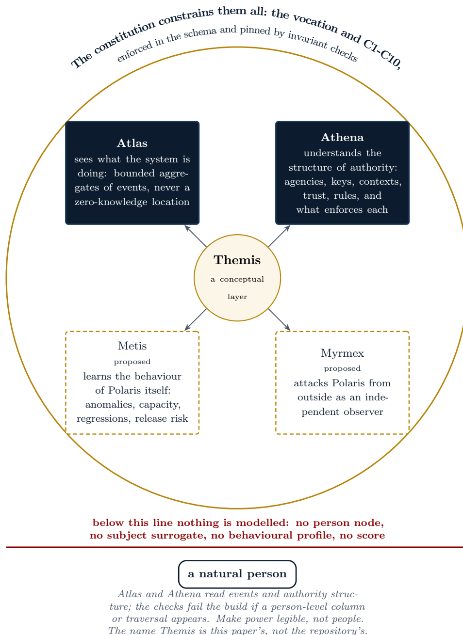
Figure 12: The cognitive layers. Atlas sees what the system is doing; Athena understands the structure of authority; Metis, proposed, would learn the behaviour of Polaris itself; Myrmex, proposed in this paper, would attack it from outside. The constitution constrains all of them. The red line is the person-prohibition: nothing above it models a natural person, and check_athena_no_person fails the build if a person-level column or traversal appears in the authority layer.
