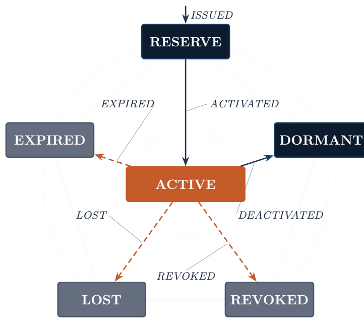
Figure 3: The token lifecycle machine, unchanged from Version 1. ACTIVE is the only operational state. A token enters at RESERVE , is activated, and leaves through one of three terminal states or into DORMANT when a successor takes over. The legal transitions are enforced by the trigger trg_token_state_machine , and every transition writes a lifecycle event automatically.
