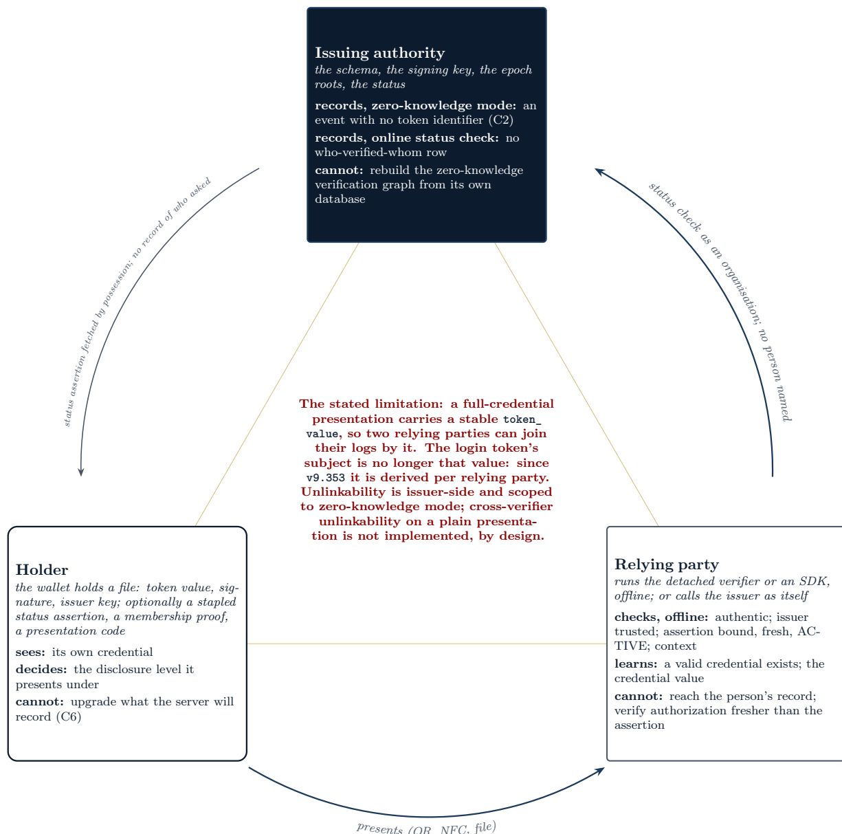
Figure 6: Holder, relying party and issuer, with what each sees and what each is prevented from seeing. The holder presents a file; the relying party decides offline with the detached verifier or an SDK and learns that a valid credential exists and its value; the issuer records, in zero-knowledge mode, an event with no token identifier, and keeps no who-verified-whom row for the online status check. The three flows form a circle turning one way; at its centre, in red, is the stated limitation: on a plain presentation the credential value is a stable handle across the verifiers it is shown to.
