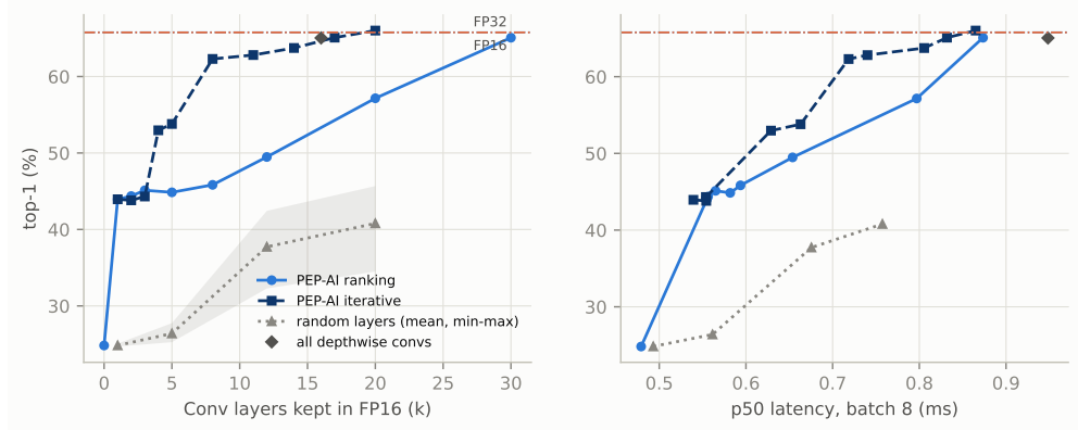
Fig. C10 Selective precision for EfficientNet-B0. Selective precision for EfficientNet-B0: top-1 accuracy versus the number of convolutions kept in FP16 (left) and versus latency at batch size 8 (right) for the PEP-AI ranking, the iterative PEP-AI ranking, random subsets (mean and range over three seeds) and all depthwise convolutions. Dash-dotted lines: FP32 and FP16.
