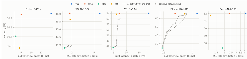
Fig. C4 Accuracy versus latency. Accuracy against the median latency at batch size 8 for FP32, FP16, INT8 and FP8 (final benchmark) and for the selective-precision INT8 variants (grey; one-shot and iterative PEP-AI ranking, shorter timing protocol).
