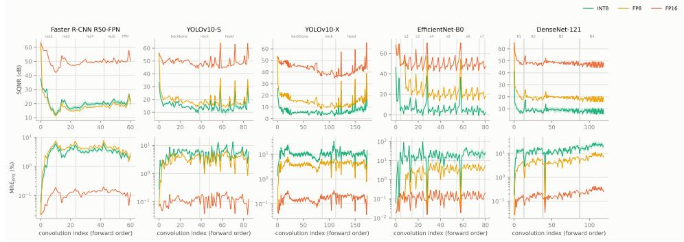
Fig. 10 Layer-wise propagation of quantization deviation. Layer-wise propagation of quantization deviation: SQNR (top) and median relative error of the channel-max projection (bottom) of every convolution, ordered by depth, for INT8 (median over 500 images, band: interquartile range), FP8 (100 images) and FP16 (500 images; Faster R-CNN 100). Grey lines and labels: network stages.
