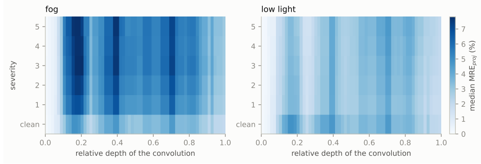
Fig. C9 Deviation of Faster R-CNN under fog and low light. Median MRE_{proj} of every INT8 Faster R-CNN convolution (backbone and FPN, ordered by depth) as a function of the severity of fog and low light, on a shared colour scale (the same 100 images at every severity; INT8 with FP32 fallback).
