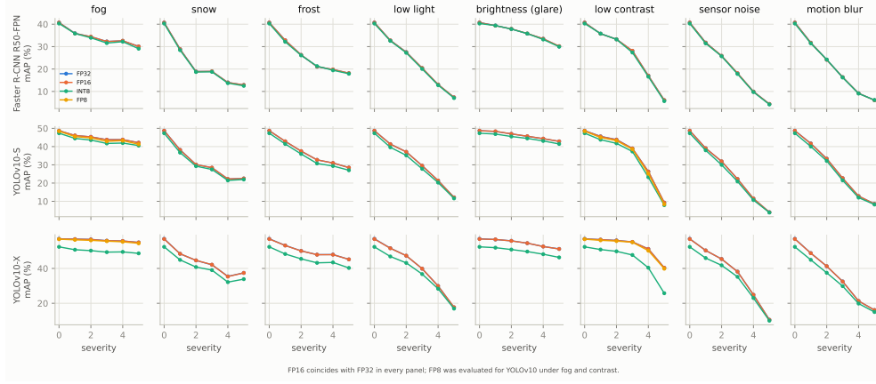
Fig. C7 Detection accuracy under adverse conditions. Box mAP of the FP32, FP16, INT8 and FP8 detectors under the eight adverse conditions at severities 0 (clean) to 5 (500 COCO val2017 images; FP8 evaluated for YOLOv10 under fog and contrast). FP16 coincides with FP32 in every panel, and FP8 stays close to FP32 (Supplementary Section B.5).
