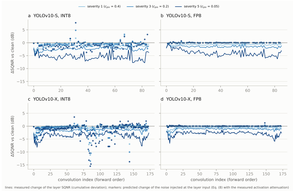
Fig. C8 Test of the static-scale prediction. Test of the static-scale prediction under reduced contrast for YOLOv10-S and YOLOv10-X in INT8 (with FP32 fallback) and FP8. Lines: measured change of the SQNR of every convolution output relative to the clean images (median over the same 100 images; cumulative deviation). Markers: change of the noise injected at the input quantizer of each convolution, computed exactly from FP32 activations and the calibrated scales (32 images), i.e. Eq. (8) with the measured activation attenuation.
