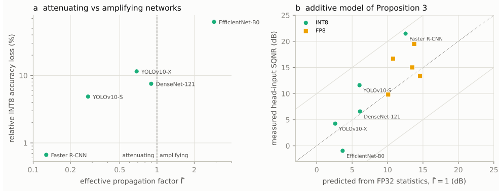
Fig. C3 Validation of the additive noise model. a Relative INT8 accuracy loss against the effective propagation factor \bar{\Gamma} of Eq. (16); networks left of the dashed line attenuate the injected noise, those right of it amplify it. b Head-input SQNR predicted from FP32 statistics with unit propagation factors against the measured value for INT8 and FP8 (dotted: identity; grey: \pm 10 dB).
