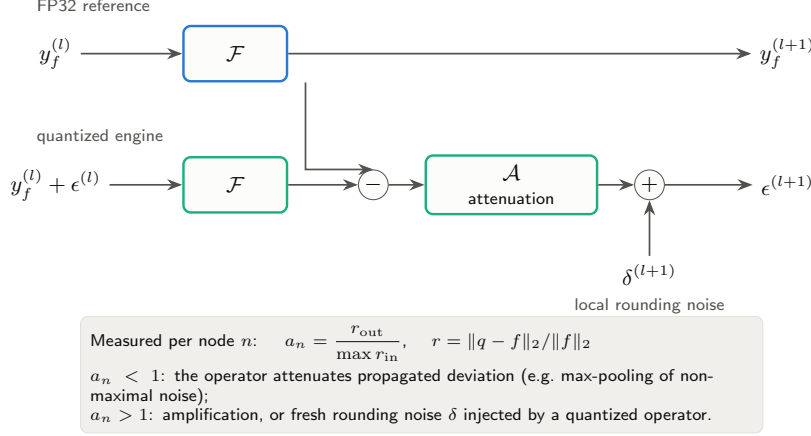
Fig. 4 Error propagation model. Error propagation model of the conference paper (Eq. 9) and the per-node amplification ratio used to estimate the attenuation operator \mathcal{A} from measured activations.
