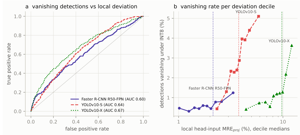
Fig. C6 Local deviation as a predictor of vanishing detections. Local head-input deviation as a predictor of detections that vanish under INT8, i.e. FP32 detections above the 0.5 threshold without an INT8 counterpart down to a score of 0.3 (COCO val2017, 5 000 images, INT8 with FP32 fallback). a ROC curves of the median MRE proj inside the detection box. b Share of vanishing detections per decile of the local deviation; dashed lines: data-derived threshold of each architecture (maximum Youden index).
