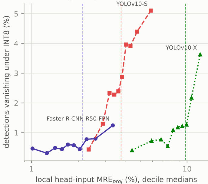
b vanishing rate per deviation decile
