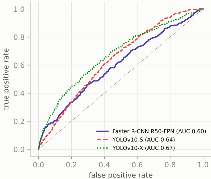
a vanishing detections vs local deviation
