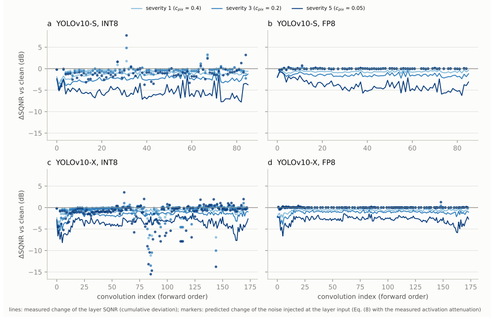
Fig. C12 Test of the static-scale prediction under reduced contrast. YOLOv10-S and YOLOv10-X in INT8 (FP32 fallback) and FP8. Lines: measured change of the SQNR of every convolution output relative to the clean images (median over the same 100 images; cumulative deviation). Markers: change of the noise injected at the input quantizer of each convolution, computed exactly from FP32 activations and the calibrated scales (32 images), i.e. Eq. (8) with the measured activation attenuation.
