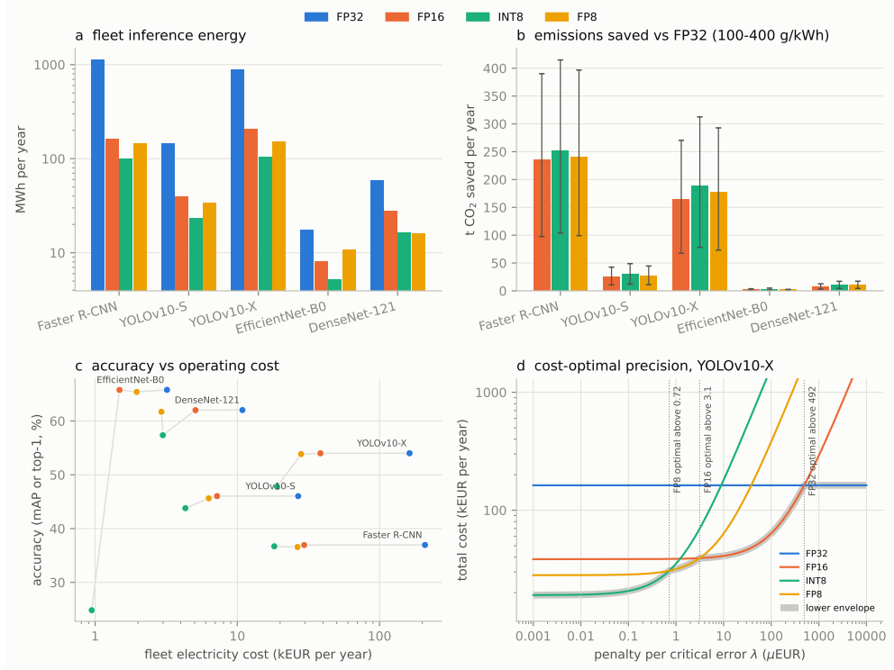
Fig. 12 AIBO fleet scenario. 1000 vehicles, six cameras at 10Hz, 16h/day, measured energy at batch size 6, i.e. the synchronised frames of the six cameras. a Annual inference energy per precision. b CO 2 saved relative to FP32 (bars: 242 g/kWh; whiskers: 100–400 g/kWh). c Task accuracy against annual electricity cost. d Total annual cost of Eq. (19) for YOLOv10-X as a function of the penalty per critical error; the grey lower envelope marks the cost-optimal precision.
