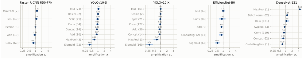
Fig. C5 Measured amplification ratio a_n per operator type. Dot: median over the nodes of each type; bar: interquartile range. Values left of the dashed line indicate attenuation of the propagated deviation.
