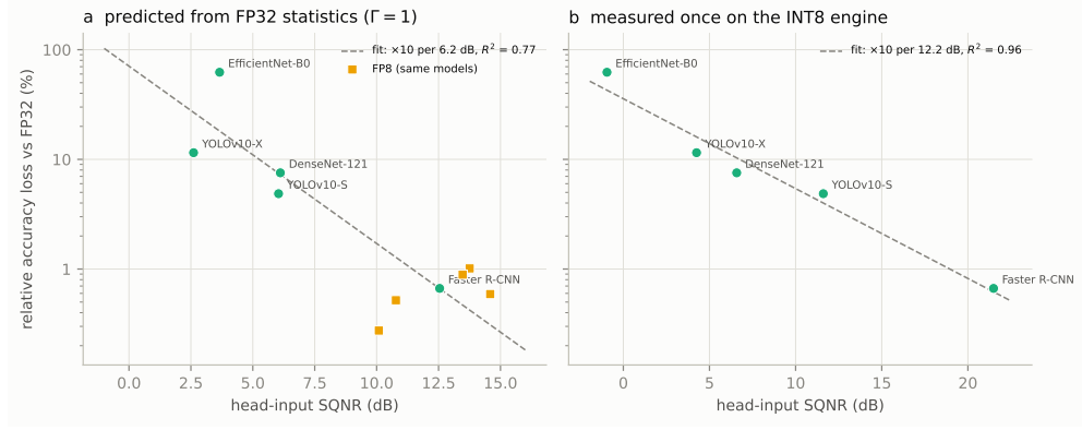
Fig. 9 Prediction of INT8 tolerance. Relative INT8 accuracy loss of the five networks against the head-input SQNR predicted from FP32 statistics with unit propagation factors ( a ; squares: FP8 engines of the same networks) and measured once on the INT8 engine with FP32 fallback ( b ); dashed: log-linear least-squares fits.
