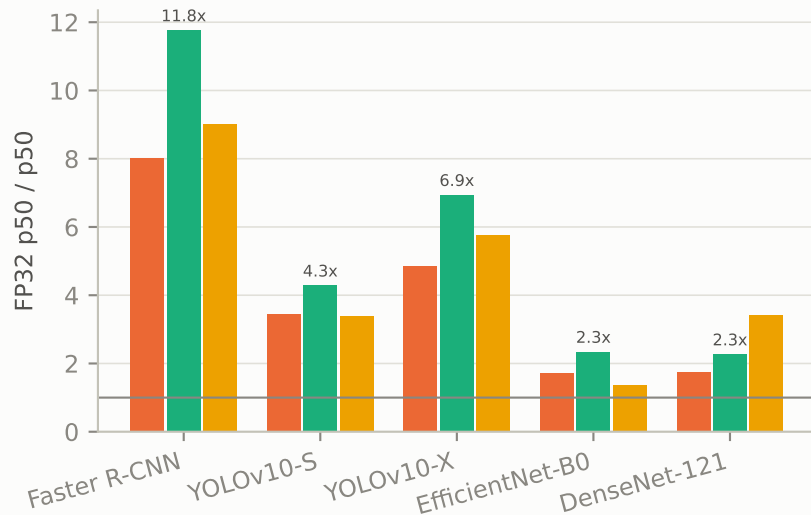
b speed-up over strict FP32, batch 8
