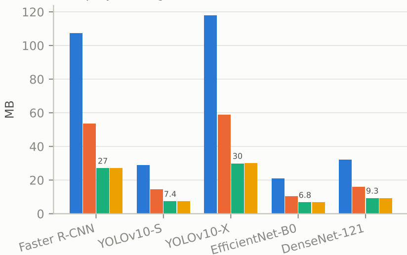
c deployed weight size
