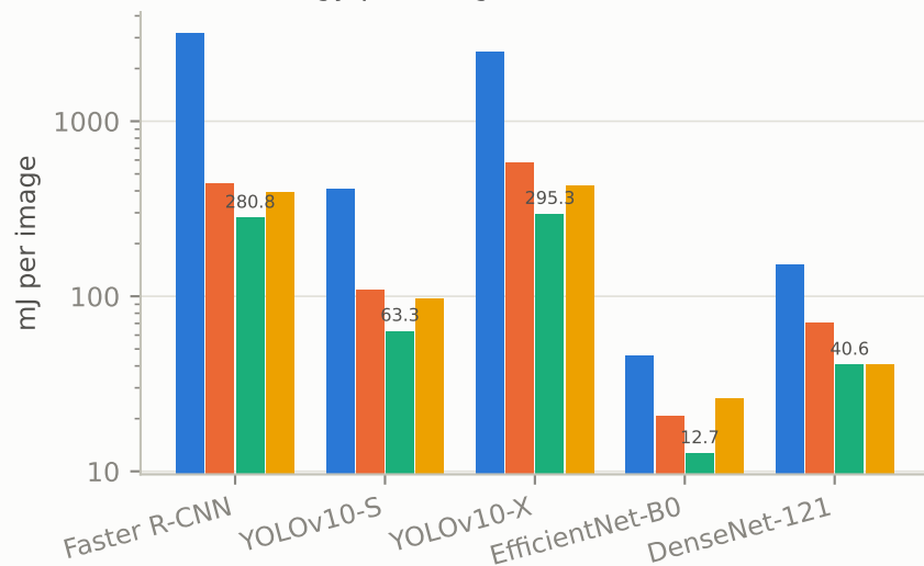
d GPU energy per image, batch 8
