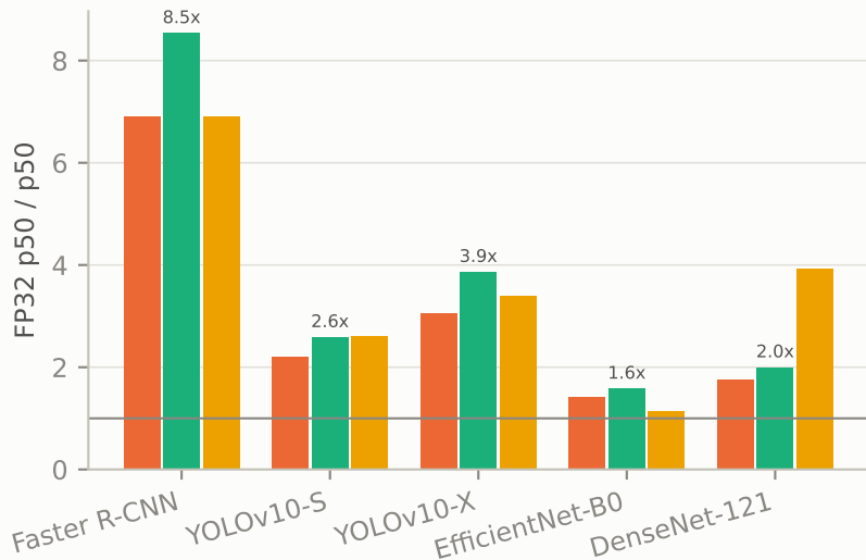
a speed-up over strict FP32, batch 1
