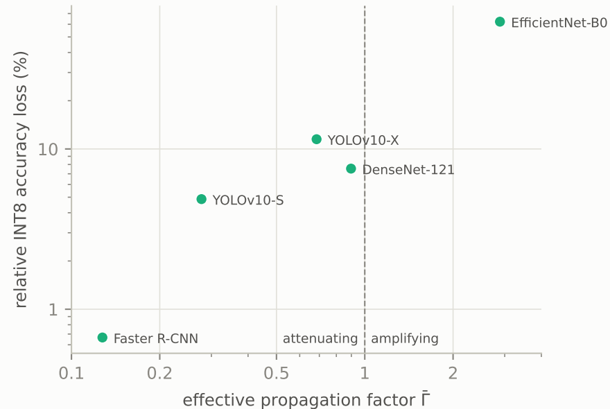
a attenuating vs amplifying networks
