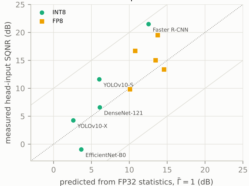
b additive model of Proposition 1
