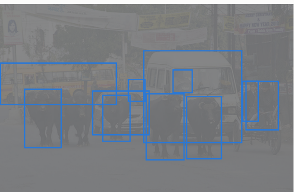
FP32, low contrast (severity 4): 11 detections
