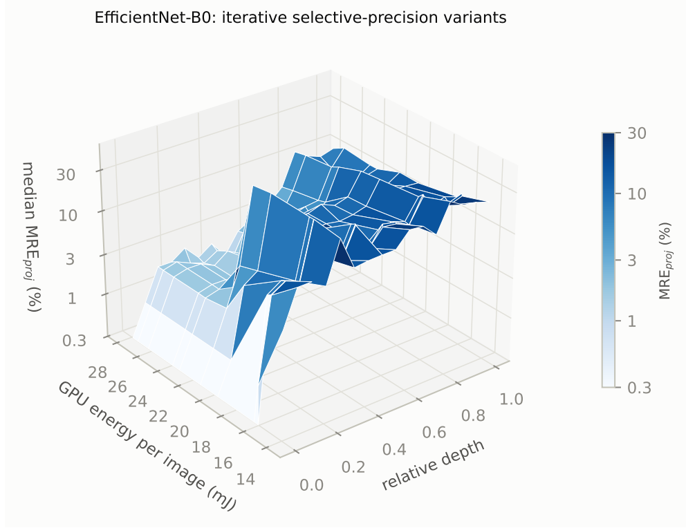
Fig. 11 Deviation, depth and energy of selective-precision variants of EfficientNet-B0. Deviation, depth and energy of the selective-precision variants of EfficientNet-B0: median MRE_{proj} of every convolution (64 calibration images) against its relative depth and the measured GPU energy per image of the variant (batch size 8; shorter protocol without CUDA graphs, comparable only between variants), for the fully quantized engine and the variants of the iterative ranking ( k = 1 –20 convolutions in FP16; 64 analysis images per variant). Logarithmic vertical axis and colour scale; depth in 16 bins. Top-1 accuracy of the variants: Table C14.
