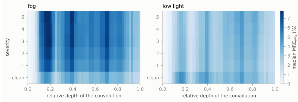
Fig. C10 Deviation of Faster R-CNN under fog and low light. Median \text{MRE}_{\text{proj}} of every INT8 Faster R-CNN convolution (backbone and FPN, ordered by depth) as a function of the severity of fog and low light, on a shared colour scale (the same 100 images at every severity; INT8 with FP32 fallback).
