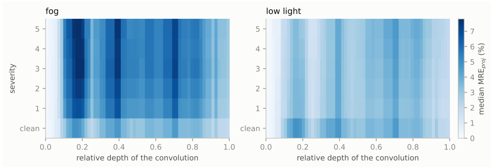
Fig. C9 Deviation of Faster R-CNN under fog and low light. Median \text{MRE}_{\text{proj}} of every INT8 Faster R-CNN convolution (backbone and FPN, ordered by depth) as a function of the severity of fog and low light, on a shared colour scale (the same 100 images at every severity; INT8 with FP32 fallback).
