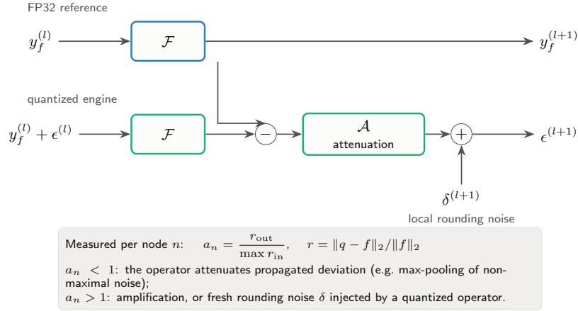
Fig. C2 Error propagation model of the conference paper. Model of Eq. 9 and the per-node amplification ratio used to estimate the attenuation operator \mathcal{A} from measured activations.
