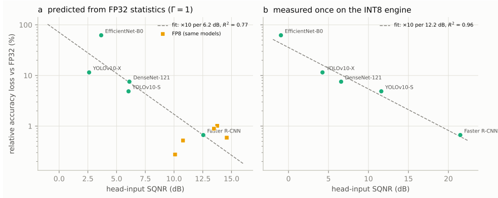
Fig. C6 Prediction of INT8 tolerance. Relative INT8 accuracy loss of the five networks against the head-input SQNR predicted from FP32 statistics with unit propagation factors (a; squares: FP8 engines of the same networks) and measured once on the INT8 engine with FP32 fallback (b); dashed: log-linear least-squares fits.
