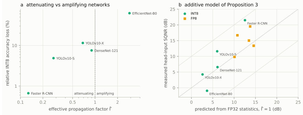
Fig. C7 Validation of the additive noise model. a Relative INT8 accuracy loss against the effective propagation factor \bar{\Gamma} of Eq. (16); networks left of the dashed line attenuate the injected noise, those right of it amplify it. b Head-input SQNR predicted from FP32 statistics with unit propagation factors against the measured value for INT8 and FP8 (dotted: identity; grey: \pm 10 dB).
