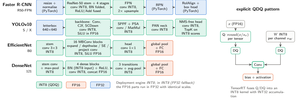
Fig. C1 Precision of the deployed INT8 engines. Precision of each architectural stage (left) and the explicit quantize–dequantize pattern that TensorRT fuses into integer kernels (right). Pre-processing and the Faster R-CNN proposal and ROI heads are not part of the quantized engine.
