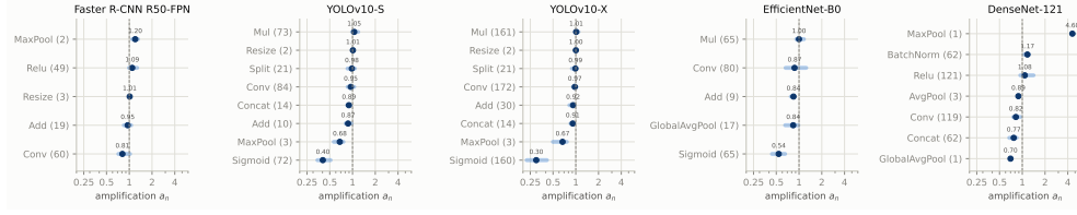
Fig. C4 Measured amplification ratio a_n per operator type. Dot: median over the nodes of each type; bar: interquartile range. Values left of the dashed line indicate attenuation of the propagated deviation.
