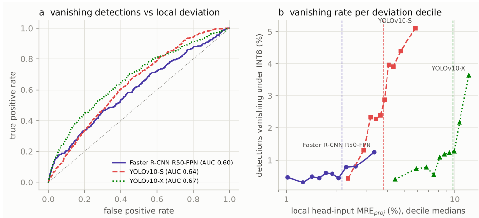
Fig. C10 Local deviation as a predictor of vanishing detections. Vanishing detections are FP32 detections above the 0.5 threshold without an INT8 counterpart down to a score of 0.3 (COCO val2017, 5000 images, INT8 with FP32 fallback). a ROC curves of the median MRE_{proj} inside the detection box. b Share of vanishing detections per decile of the local deviation; dashed lines: data-derived threshold of each architecture (maximum Youden index).
