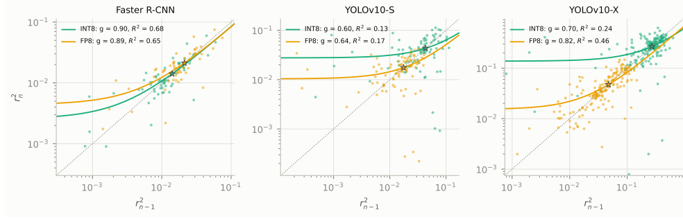
Fig. C5 Layer-to-layer recursion of the relative error. Layer-to-layer map of the relative error power r_{n-1}^2 \mapsto r_n^2 over consecutive convolutions (medians over the analysis images) for INT8 and FP8, with the least-squares fit of r_n^2 = g^2 r_{n-1}^2 + \rho^2 and its fixed point (star, Eq. (15)) on the identity line (dotted).
