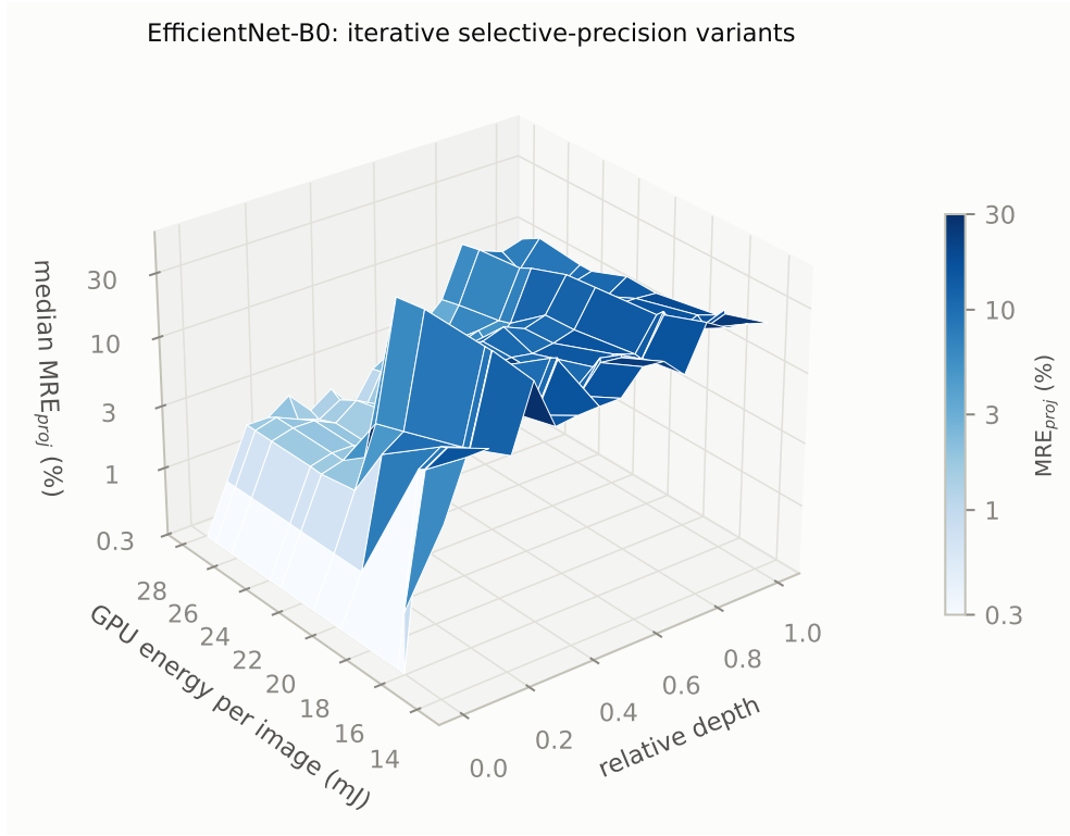
Fig. 8 Deviation, depth and energy of selective-precision variants of EfficientNet-B0. Median MRE_{proj} of every convolution against its relative depth (16 bins) and the GPU energy per image of the variant, for the fully quantized engine and the iterative ranking with k = 1-20 convolutions in FP16 (64 images each; batch size 8, shorter protocol without CUDA graphs, comparable only between variants). Logarithmic vertical axis and colour scale; top-1 accuracy in Table C15.
