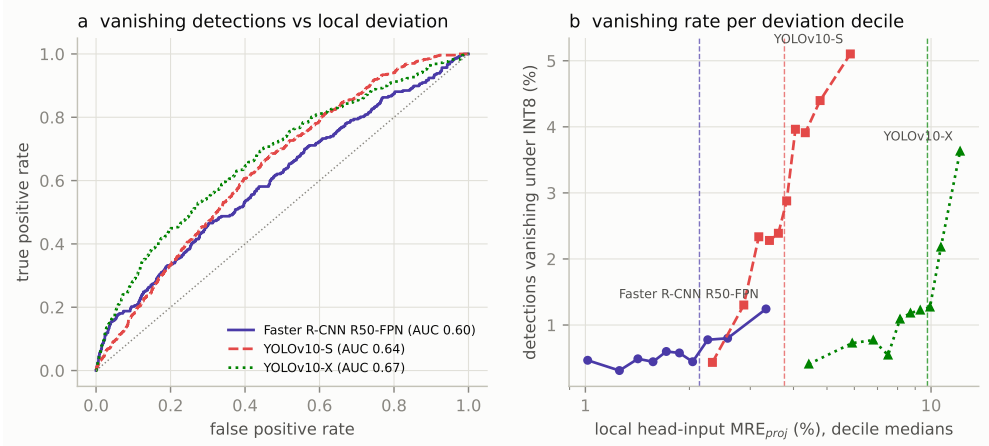
Fig. C11 Local deviation as a predictor of vanishing detections. Vanishing detections are FP32 detections above the 0.5 threshold without an INT8 counterpart down to a score of 0.3 (COCO val2017, 5000 images, INT8 with FP32 fallback). a ROC curves of the median MRE_{proj} inside the detection box. b Share of vanishing detections per decile of the local deviation; dashed lines: data-derived threshold of each architecture (maximum Youden index).
