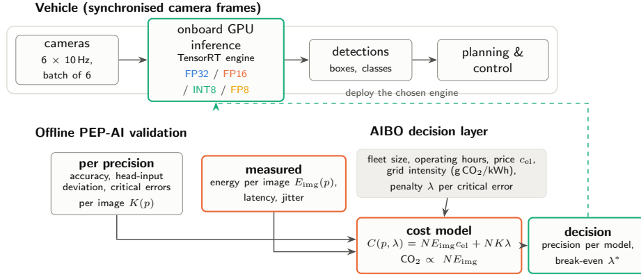
Fig. C1 AIBO view of quantized perception. Offline PEP-AI validation supplies accuracy, deviation, the critical errors per image K(p) and the measured energy per image E_{\text{img}}(p) of every precision; combined with fleet parameters, electricity price, grid intensity and a penalty \lambda per critical error, the cost model of Eq. (19) selects the precision of each deployed engine.
