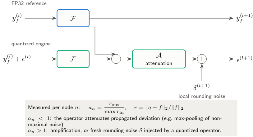
Fig. C3 Error propagation model. Model of Eq. 9 and the per-node amplification ratio used to estimate the attenuation operator \mathcal{A} from measured activations.
