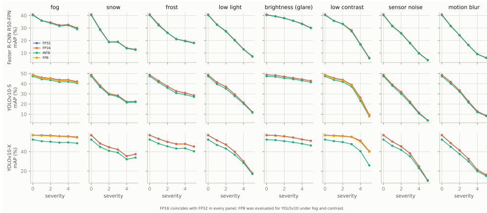
Fig. C7 Detection accuracy under adverse conditions. Box mAP of the FP32, FP16, INT8 and FP8 detectors under the eight adverse conditions at severities 0 (clean) to 5 (500 COCO val2017 images; FP8 evaluated for YOLOv10 under fog and contrast). FP16 coincides with FP32 in every panel, and FP8 stays close to FP32 (Supplementary Section B.5).
