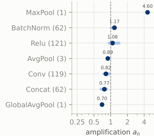
DenseNet-121
