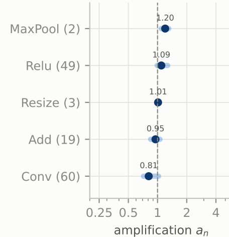
Faster R-CNN R50-FPN
