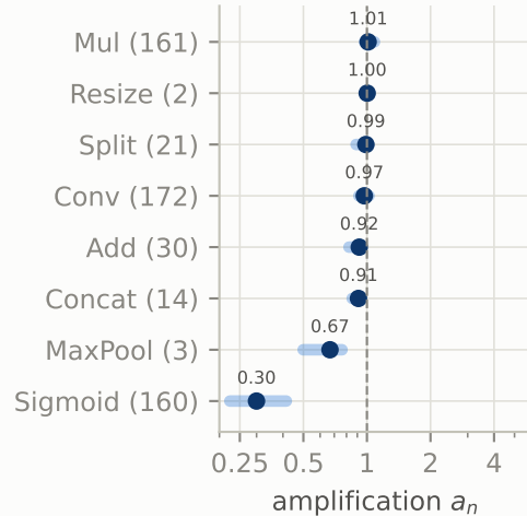
YOLOv10-X
