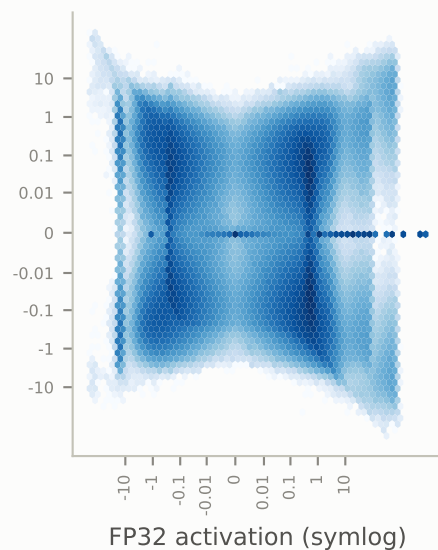
YOLOv10-X
