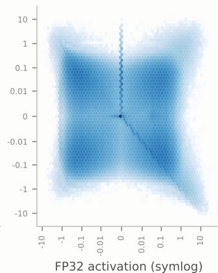
DenseNet-121
