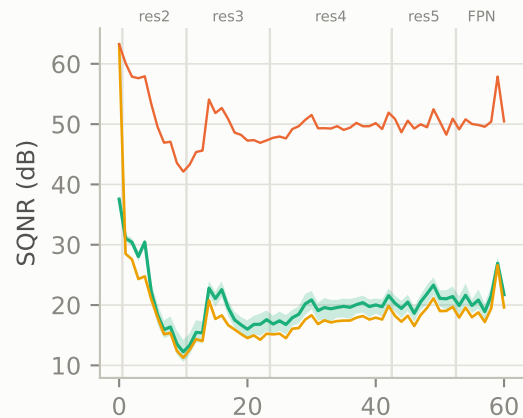
Faster R-CNN R50-FPN
