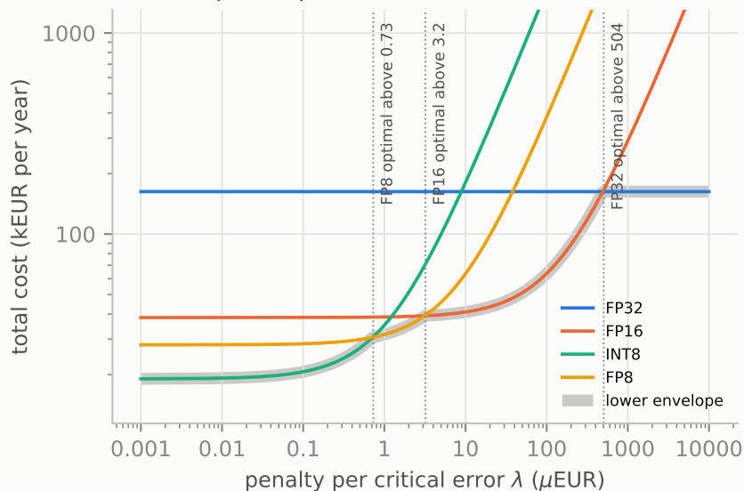
d cost-optimal precision, YOLOv10-X
