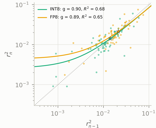
Faster R-CNN
