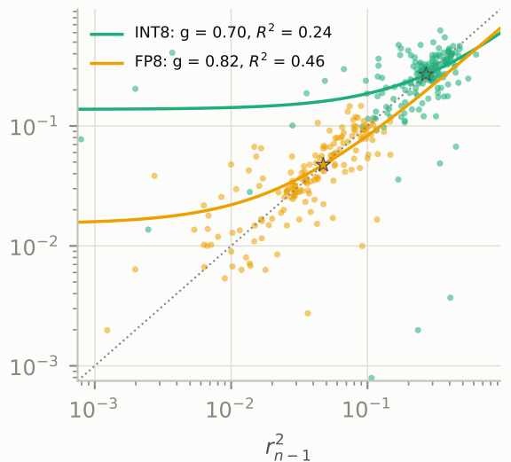
YOLOv10-X
