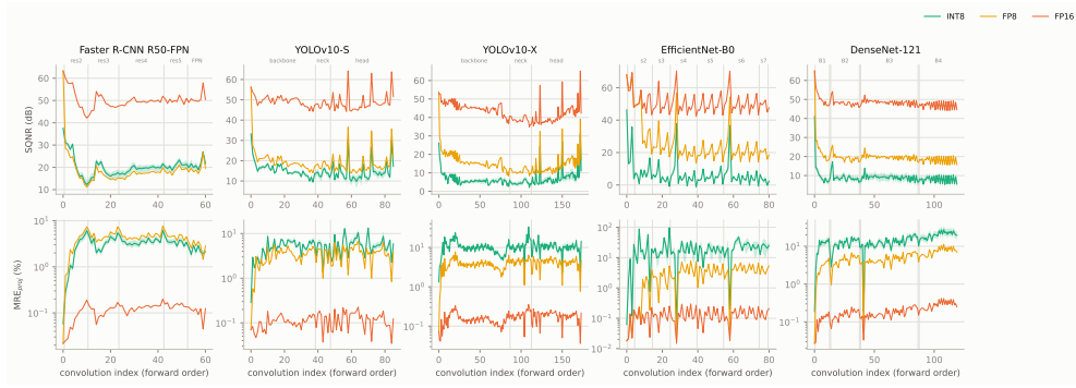
Fig. 10 Layer-wise propagation of quantization deviation. Layer-wise propagation of quantization deviation: SQNR (top) and median relative error of the channel-max projection (bottom) of every convolution, ordered by depth, for INT8 (median over 500 images, band: interquartile range), FP8 (100 images) and FP16 (500 images; Faster R-CNN 100). Grey lines and labels: network stages.
