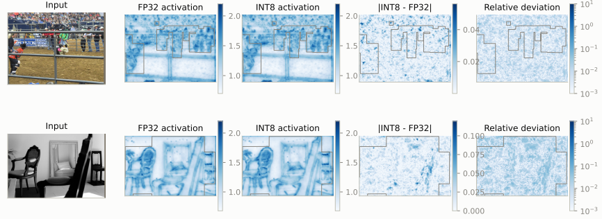
Faster R-CNN R50-FPN: channel-max activations averaged over all convolutions
