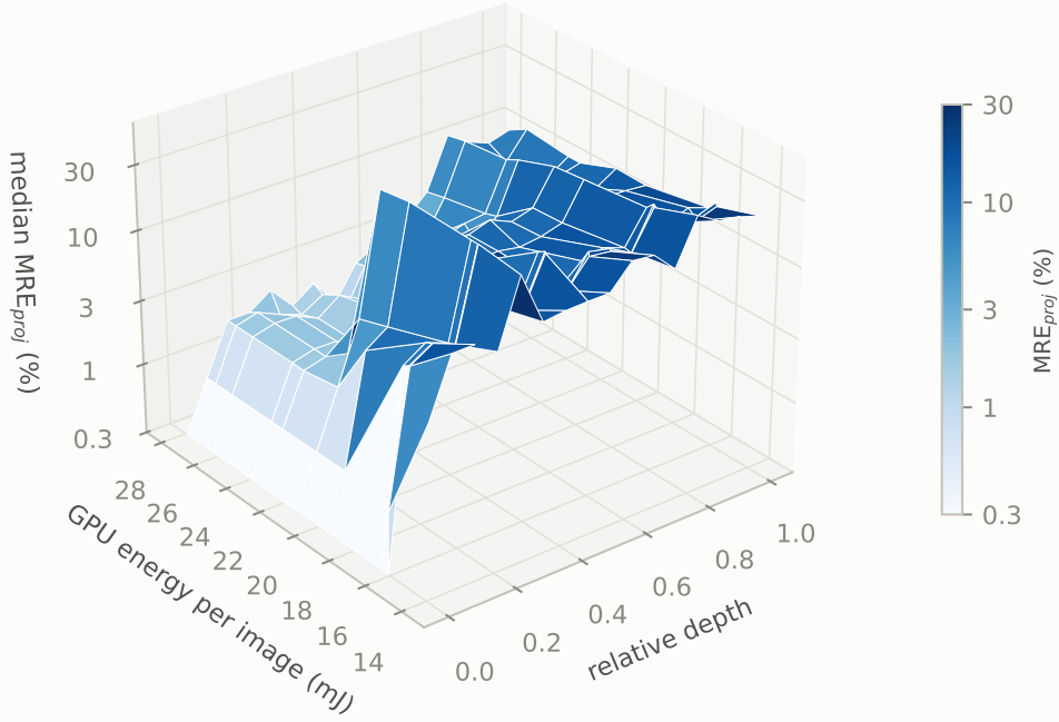
Fig. 11 Deviation, depth and energy of selective-precision variants of EfficientNet-B0. Deviation, depth and energy of the selective-precision variants of EfficientNet-B0: median MRE proj of every convolution (64 calibration images) against its relative depth and the measured GPU energy per image of the variant (batch size 8; shorter protocol without CUDA graphs, comparable only between variants), for the fully quantized engine and the variants of the iterative ranking ( k = 1-20 convolutions in FP16; 64 analysis images per variant). Logarithmic vertical axis and colour scale; depth in 16 bins. Top-1 accuracy of the variants: Table C7.
