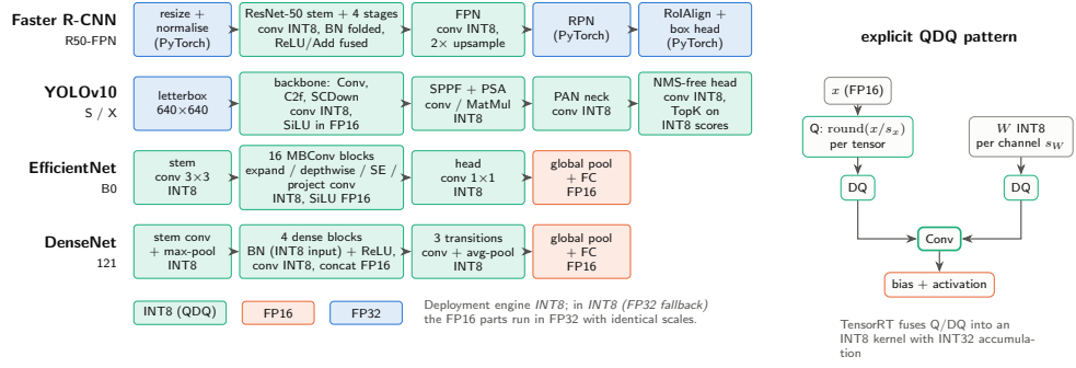
Fig. 2 Precision of the deployed INT8 engines. Precision of each architectural stage in the deployed INT8 engines (left) and the explicit quantize–dequantize pattern that TensorRT fuses into integer kernels (right). Pre-processing and the Faster R-CNN proposal and ROI heads are not part of the quantized engine.
