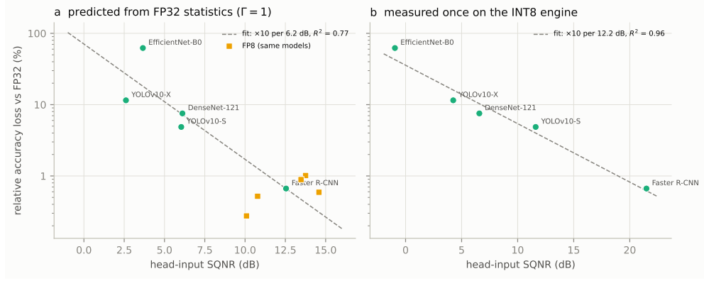
Fig. C3 Prediction of INT8 tolerance. Relative INT8 accuracy loss of the five networks against the head-input SQNR predicted from FP32 statistics with unit propagation factors (a; squares: FP8 engines of the same networks) and measured once on the INT8 engine with FP32 fallback (b); dashed: log-linear least-squares fits.
