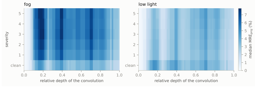
Fig. C14 Deviation of Faster R-CNN under fog and low light. Median \text{MRE}_{\text{proj}} of every INT8 Faster R-CNN convolution (backbone and FPN, ordered by depth) as a function of the severity of fog and low light, on a shared colour scale (the same 100 images at every severity; INT8 with FP32 fallback).
